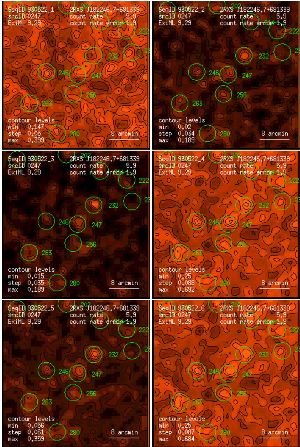
Figure 247: RASS 930522: detection 0247: band rate images, Gaussian filter: (1) PSPC channels 11 – 41, (2) 52 – 90, (3) 91 – 201, (4) 11 – 235, (5) 52 – 201, (6) 11 – 201. Broad band rates in counts/ks. Band rate contour levels in counts/ks/arcmin 2 .
