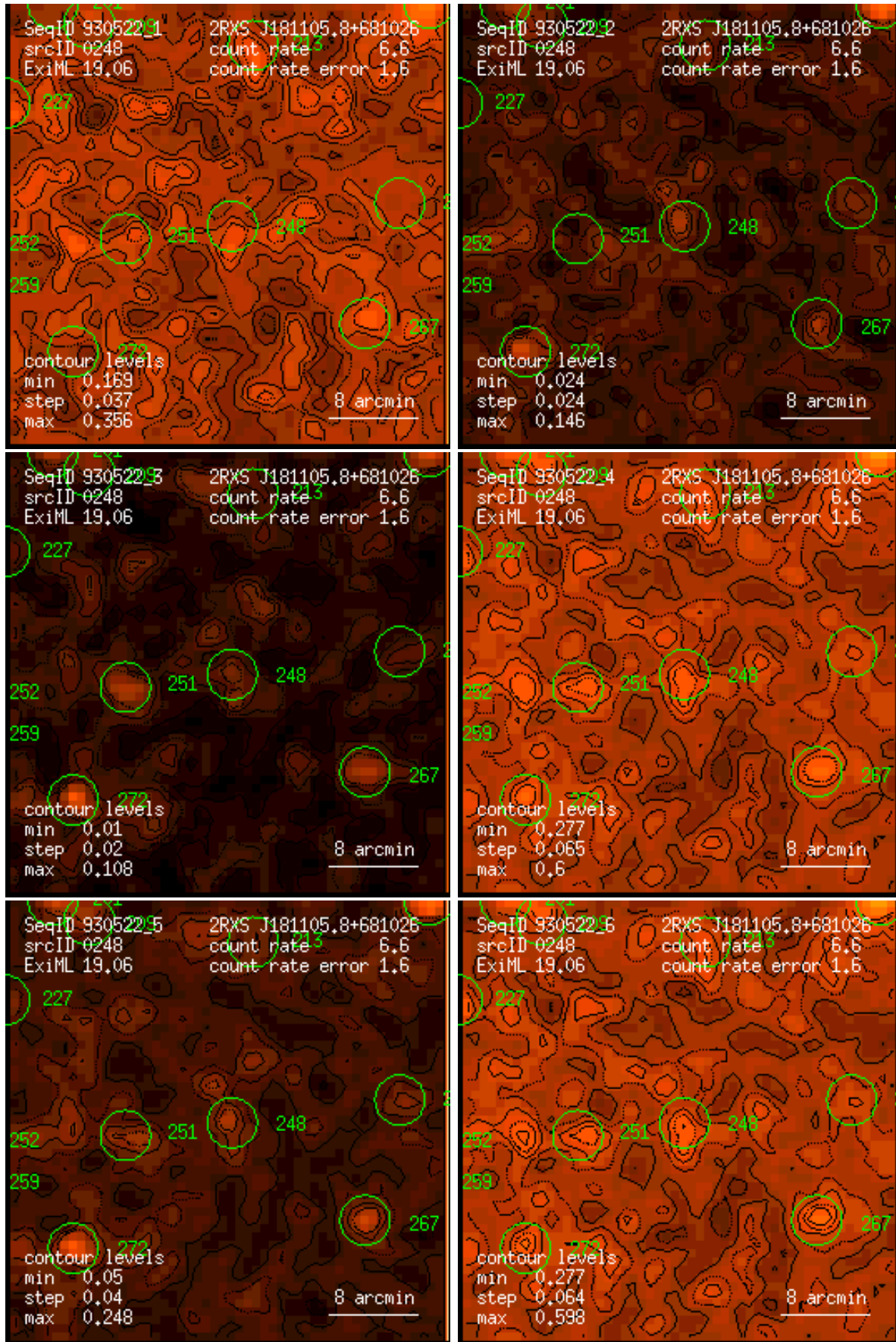
Figure 248: RASS 930522: detection 0248: band rate images, Gaussian filter: (1) PSPC channels 11 – 41, (2) 52 – 90, (3) 91 – 201, (4) 11 – 235, (5) 52 – 201, (6) 11 – 201. Broad band rates in counts/ks. Band rate contour levels in counts/ks/arcmin 2 .
