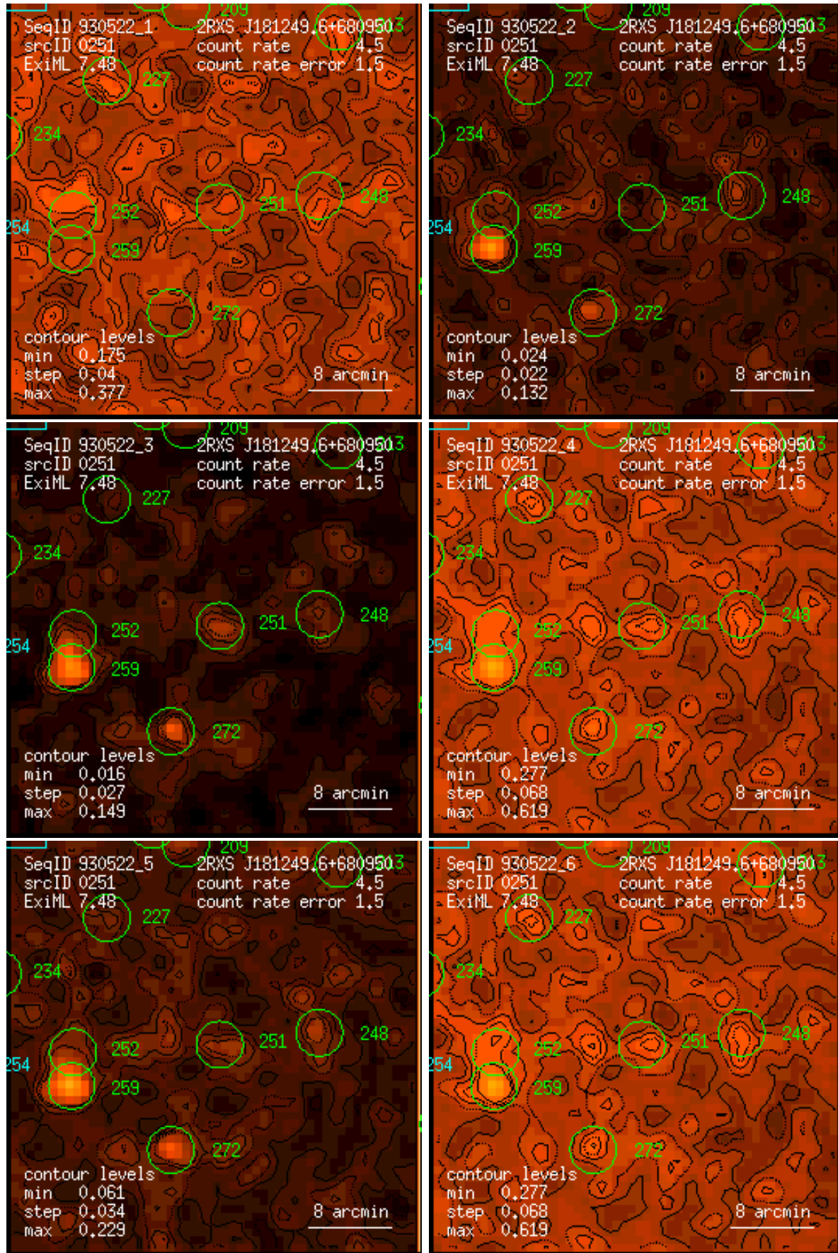
Figure 251: RASS 930522: detection 0251: band rate images, Gaussian filter: (1) PSPC channels 11 – 41, (2) 52 – 90, (3) 91 – 201, (4) 11 – 235, (5) 52 – 201, (6) 11 – 201. Broad band rates in counts/ks. Band rate contour levels in counts/ks/arcmin 2 .
