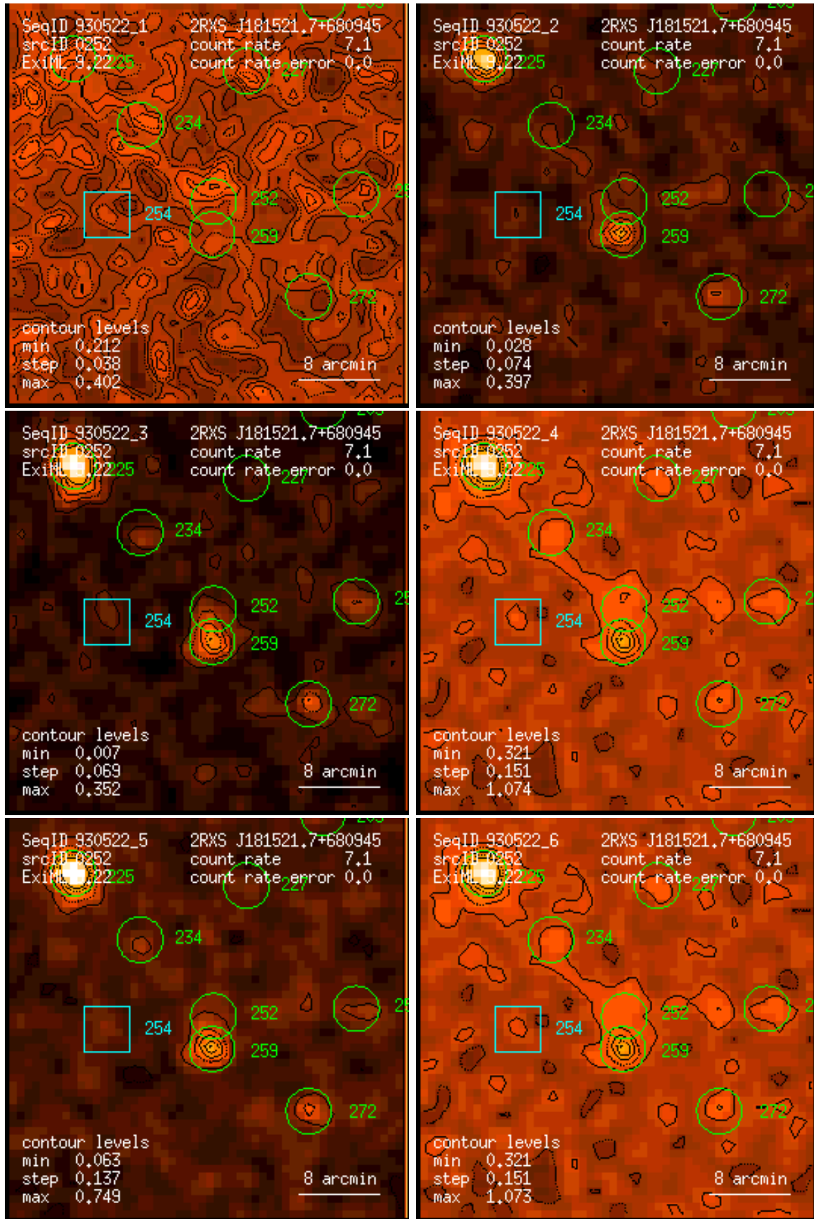
Figure 252: RASS 930522: detection 0252: band rate images, Gaussian filter: (1) PSPC channels 11 – 41, (2) 52 – 90, (3) 91 – 201, (4) 11 – 235, (5) 52 – 201, (6) 11 – 201. Broad band rates in counts/ks. Band rate contour levels in counts/ks/arcmin 2 .
