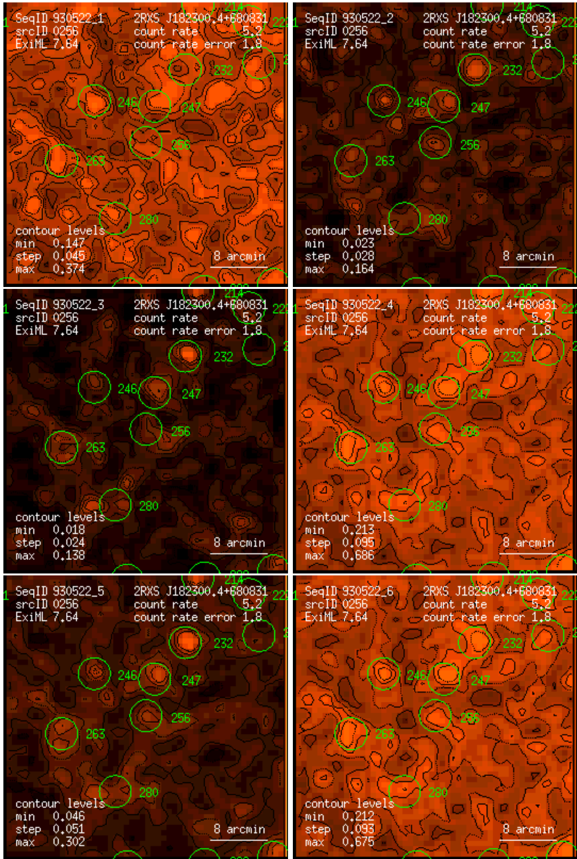
Figure 256: RASS 930522: detection 0256: band rate images, Gaussian filter: (1) PSPC channels 11 – 41, (2) 52 – 90, (3) 91 – 201, (4) 11 – 235, (5) 52 – 201, (6) 11 – 201. Broad band rates in counts/ks. Band rate contour levels in counts/ks/arcmin 2 .
