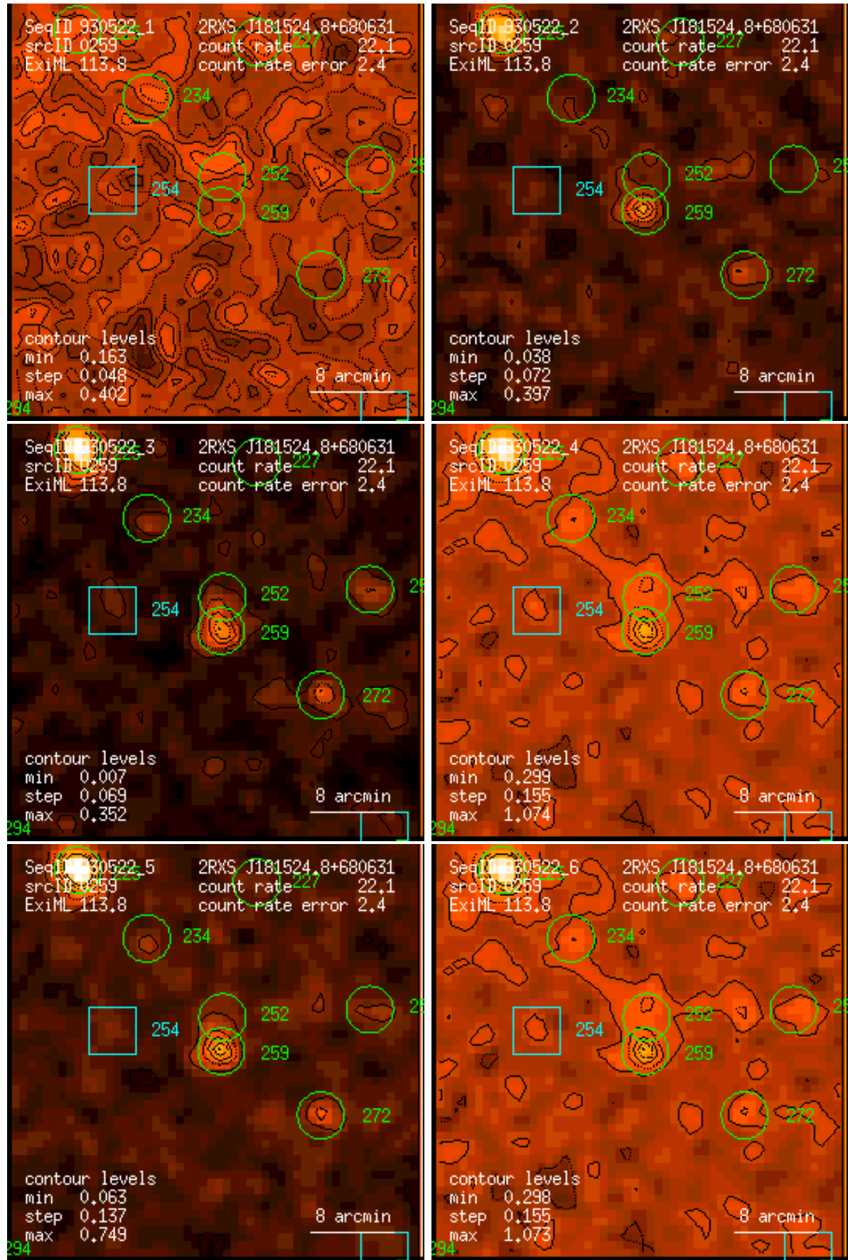
Figure 259: RASS 930522: detection 0259: band rate images, Gaussian filter: (1) PSPC channels 11 – 41, (2) 52 – 90, (3) 91 – 201, (4) 11 – 235, (5) 52 – 201, (6) 11 – 201. Broad band rates in counts/ks. Band rate contour levels in counts/ks/arcmin 2 .
