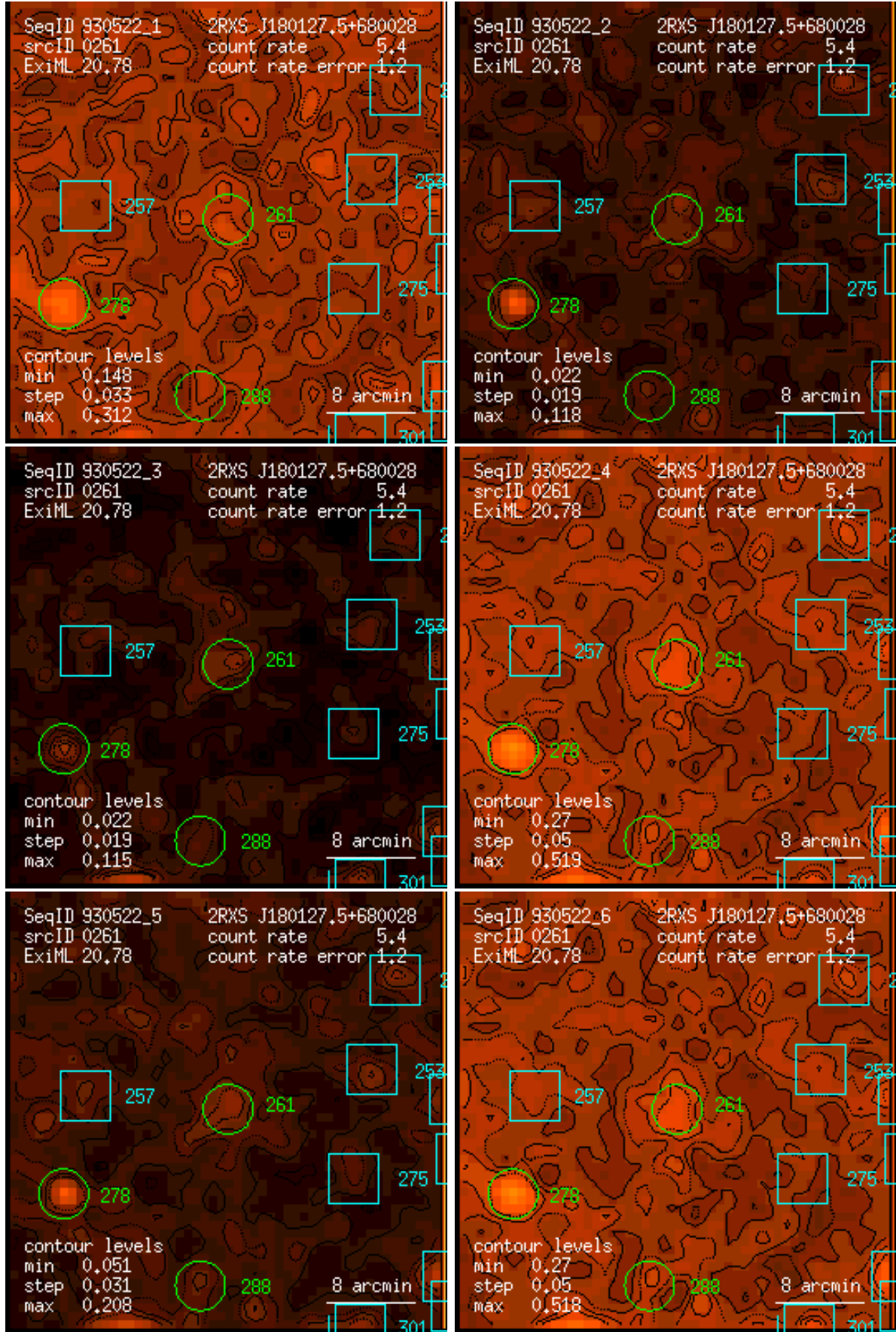
Figure 261: RASS 930522: detection 0261: band rate images, Gaussian filter: (1) PSPC channels 11 – 41, (2) 52 – 90, (3) 91 – 201, (4) 11 – 235, (5) 52 – 201, (6) 11 – 201. Broad band rates in counts/ks. Band rate contour levels in counts/ks/arcmin 2 .
