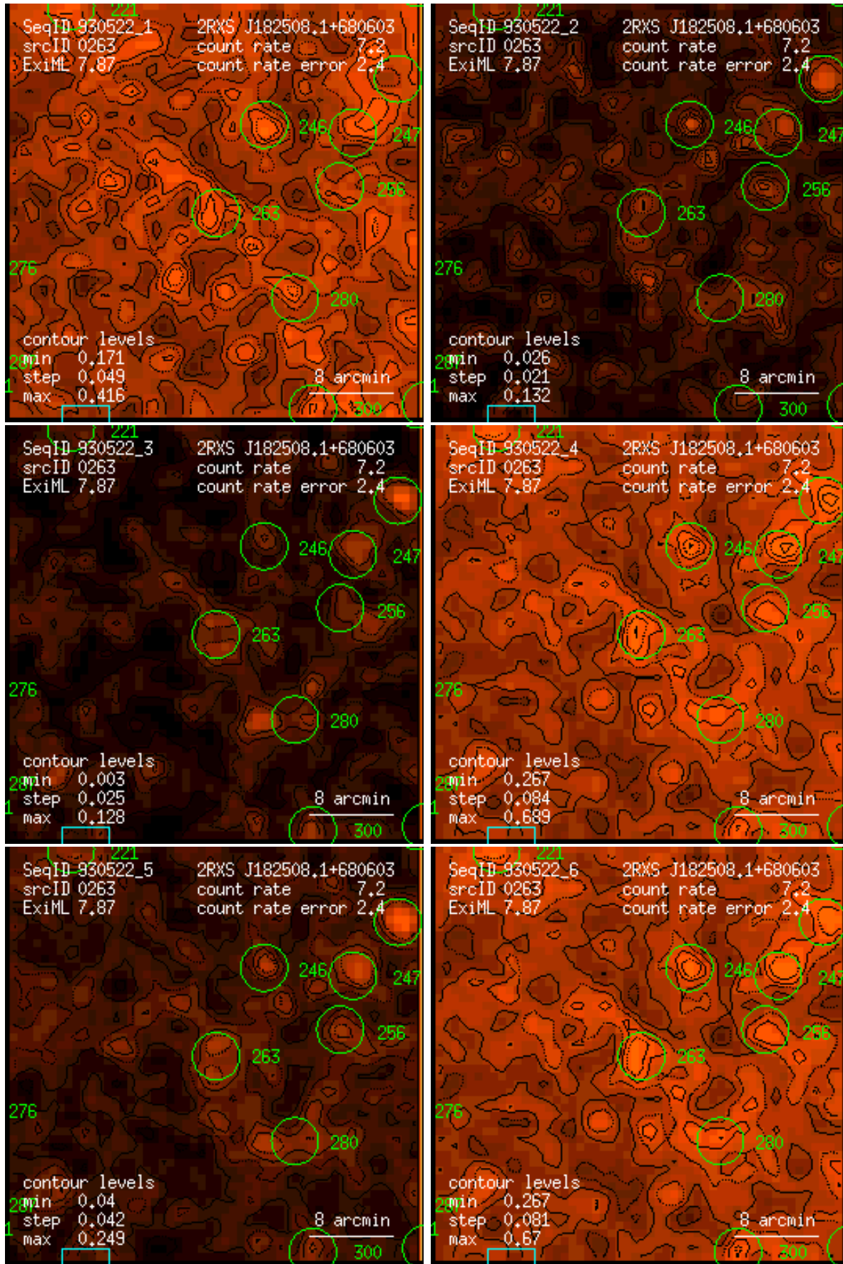
Figure 263: RASS 930522: detection 0263: band rate images, Gaussian filter: (1) PSPC channels 11 – 41, (2) 52 – 90, (3) 91 – 201, (4) 11 – 235, (5) 52 – 201, (6) 11 – 201. Broad band rates in counts/ks. Band rate contour levels in counts/ks/arcmin 2 .
