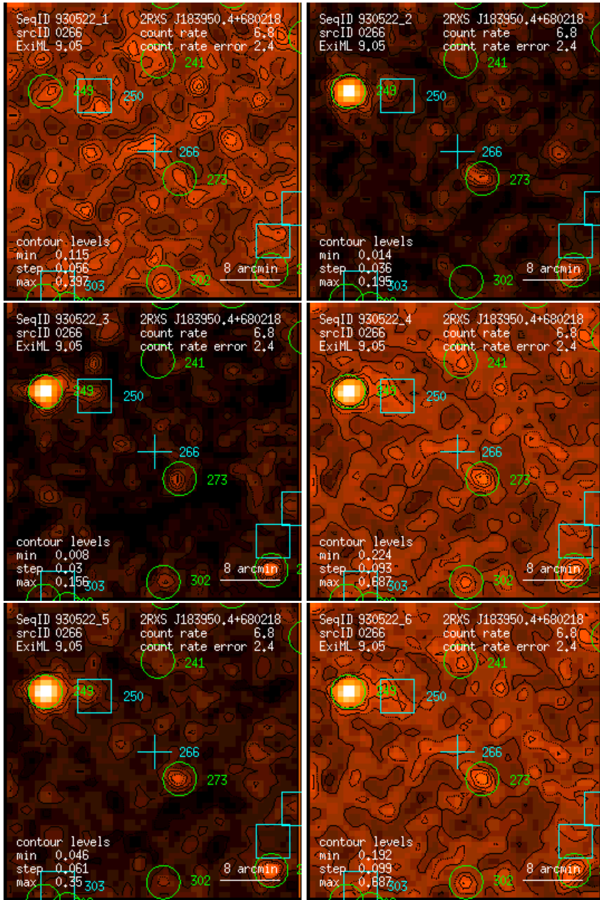
Figure 266: RASS 930522: detection 0266: band rate images, Gaussian filter: (1) PSPC channels 11 – 41, (2) 52 – 90, (3) 91 – 201, (4) 11 – 235, (5) 52 – 201, (6) 11 – 201. Broad band rates in counts/ks. Band rate contour levels in counts/ks/arcmin 2 .
