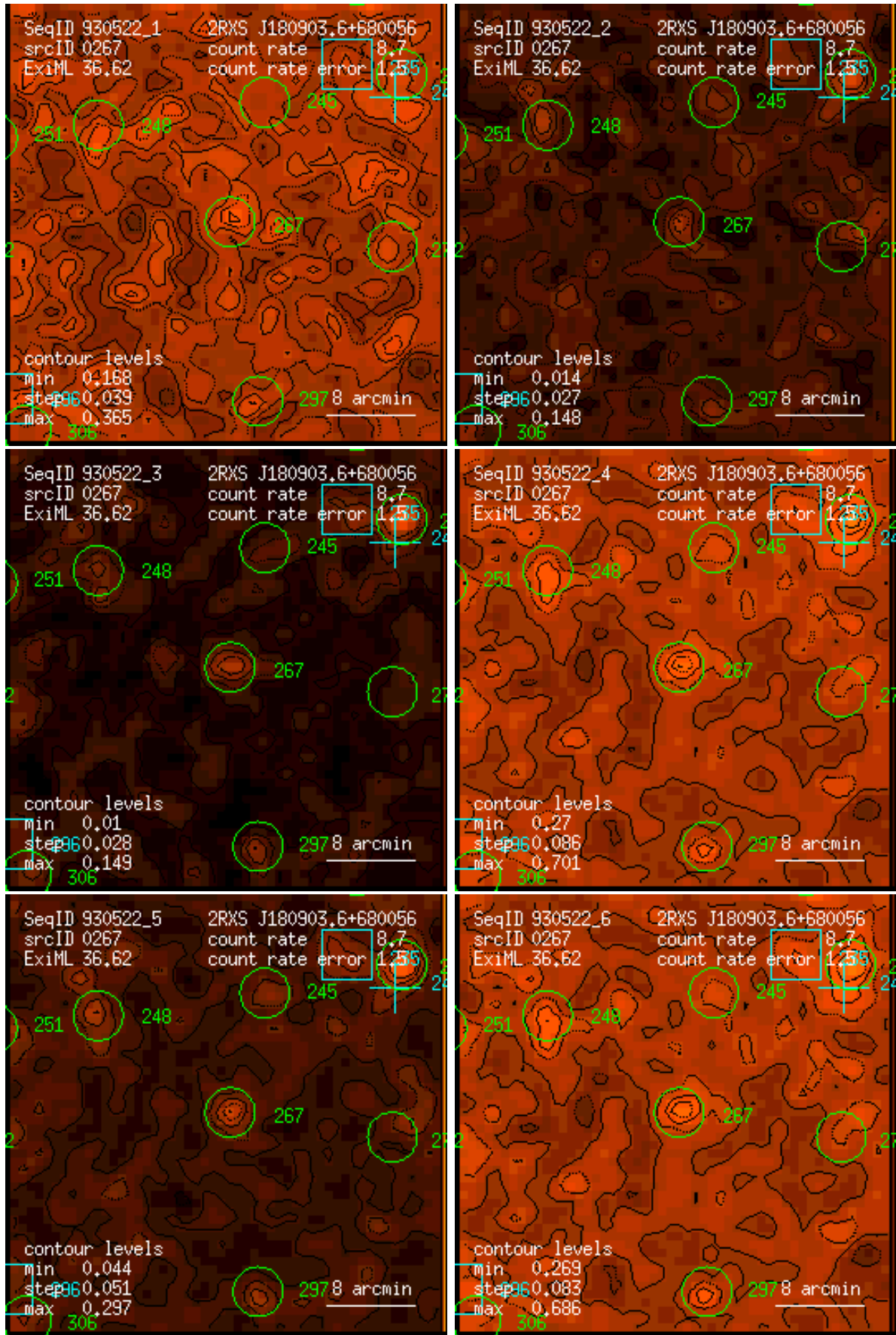
Figure 267: RASS 930522: detection 0267: band rate images, Gaussian filter: (1) PSPC channels 11 – 41, (2) 52 – 90, (3) 91 – 201, (4) 11 – 235, (5) 52 – 201, (6) 11 – 201. Broad band rates in counts/ks. Band rate contour levels in counts/ks/arcmin 2 .
