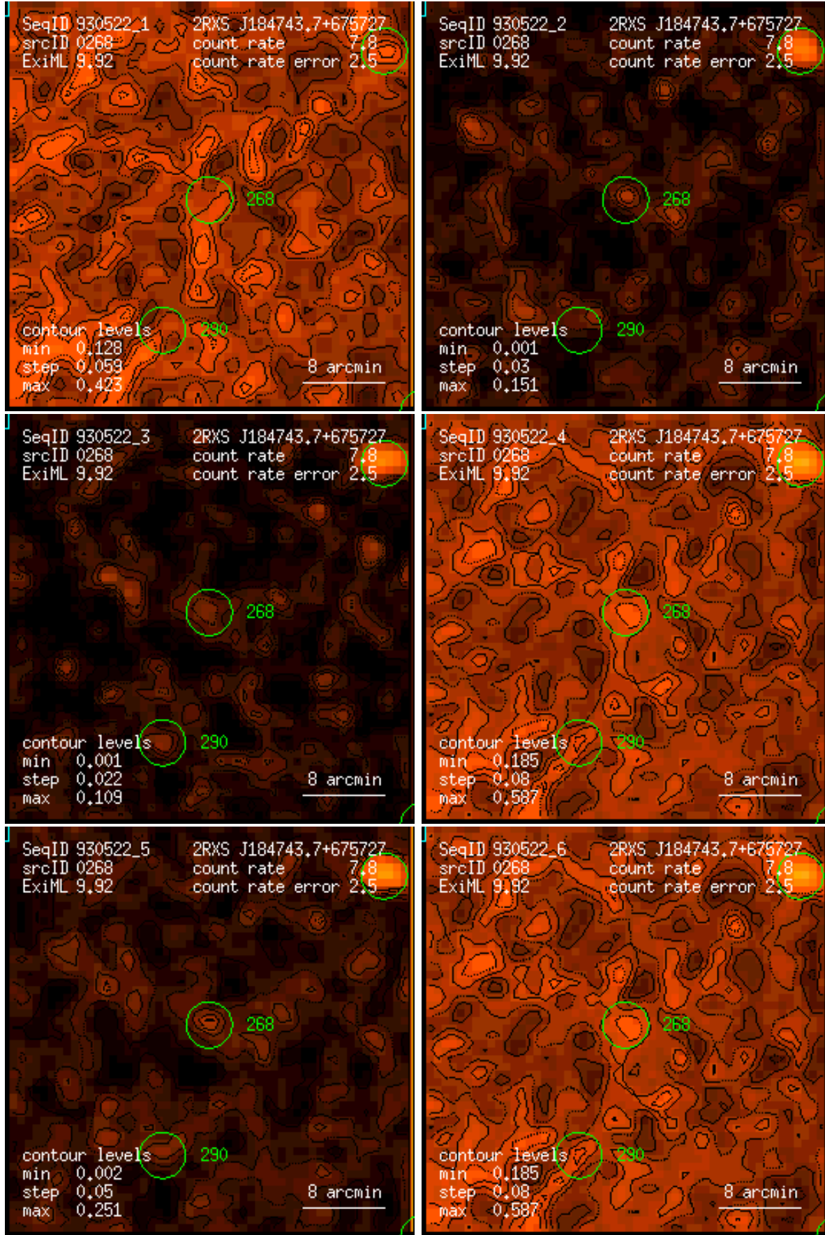
Figure 268: RASS 930522: detection 0268: band rate images, Gaussian filter: (1) PSPC channels 11 – 41, (2) 52 – 90, (3) 91 – 201, (4) 11 – 235, (5) 52 – 201, (6) 11 – 201. Broad band rates in counts/ks. Band rate contour levels in counts/ks/arcmin 2 .
