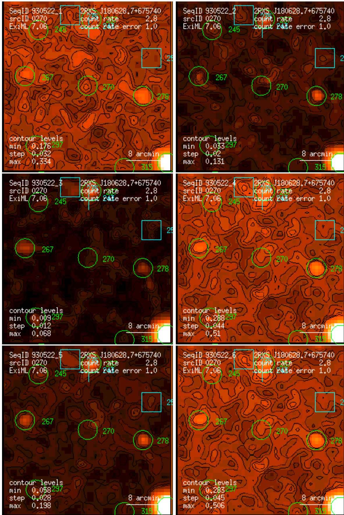
Figure 270: RASS 930522: detection 0270: band rate images, Gaussian filter: (1) PSPC channels 11 – 41, (2) 52 – 90, (3) 91 – 201, (4) 11 – 235, (5) 52 – 201, (6) 11 – 201. Broad band rates in counts/ks. Band rate contour levels in counts/ks/arcmin 2 .
