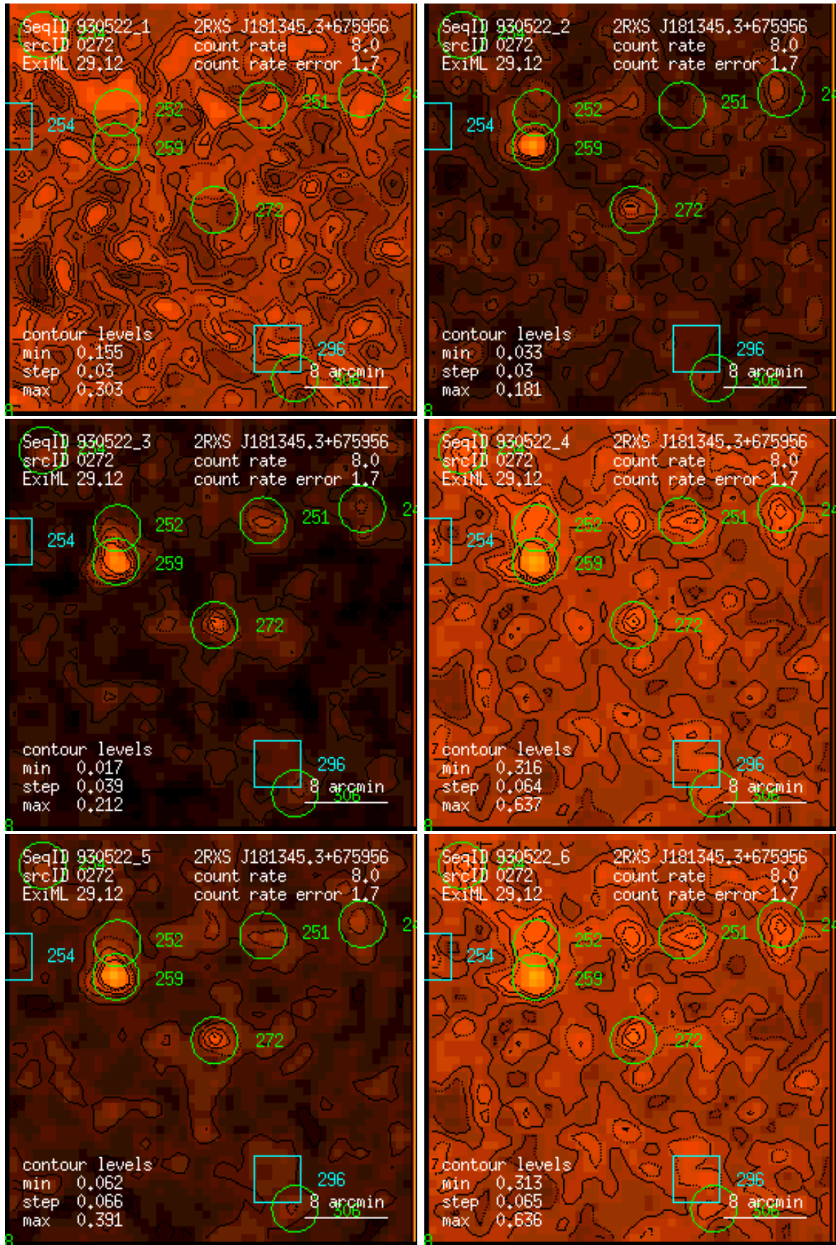
Figure 272: RASS 930522: detection 0272: band rate images, Gaussian filter: (1) PSPC channels 11 – 41, (2) 52 – 90, (3) 91 – 201, (4) 11 – 235, (5) 52 – 201, (6) 11 – 201. Broad band rates in counts/ks. Band rate contour levels in counts/ks/arcmin 2 .
