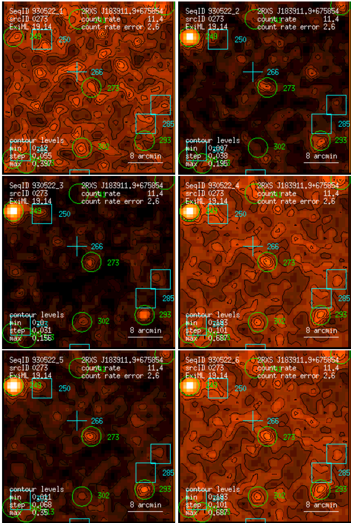
Figure 273: RASS 930522: detection 0273: band rate images, Gaussian filter: (1) PSPC channels 11 – 41, (2) 52 – 90, (3) 91 – 201, (4) 11 – 235, (5) 52 – 201, (6) 11 – 201. Broad band rates in counts/ks. Band rate contour levels in counts/ks/arcmin 2 .
