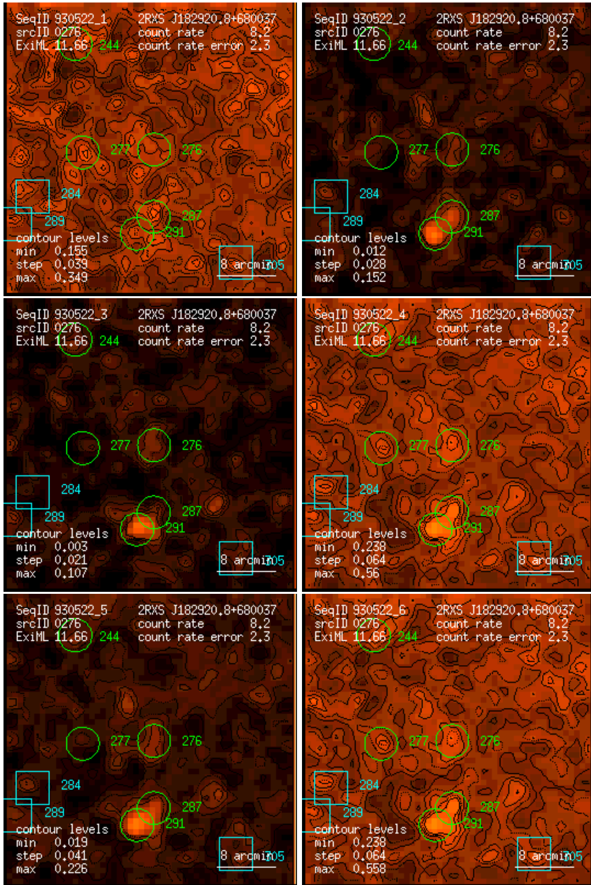
Figure 276: RASS 930522: detection 0276: band rate images, Gaussian filter: (1) PSPC channels 11 – 41, (2) 52 – 90, (3) 91 – 201, (4) 11 – 235, (5) 52 – 201, (6) 11 – 201. Broad band rates in counts/ks. Band rate contour levels in counts/ks/arcmin 2 .
