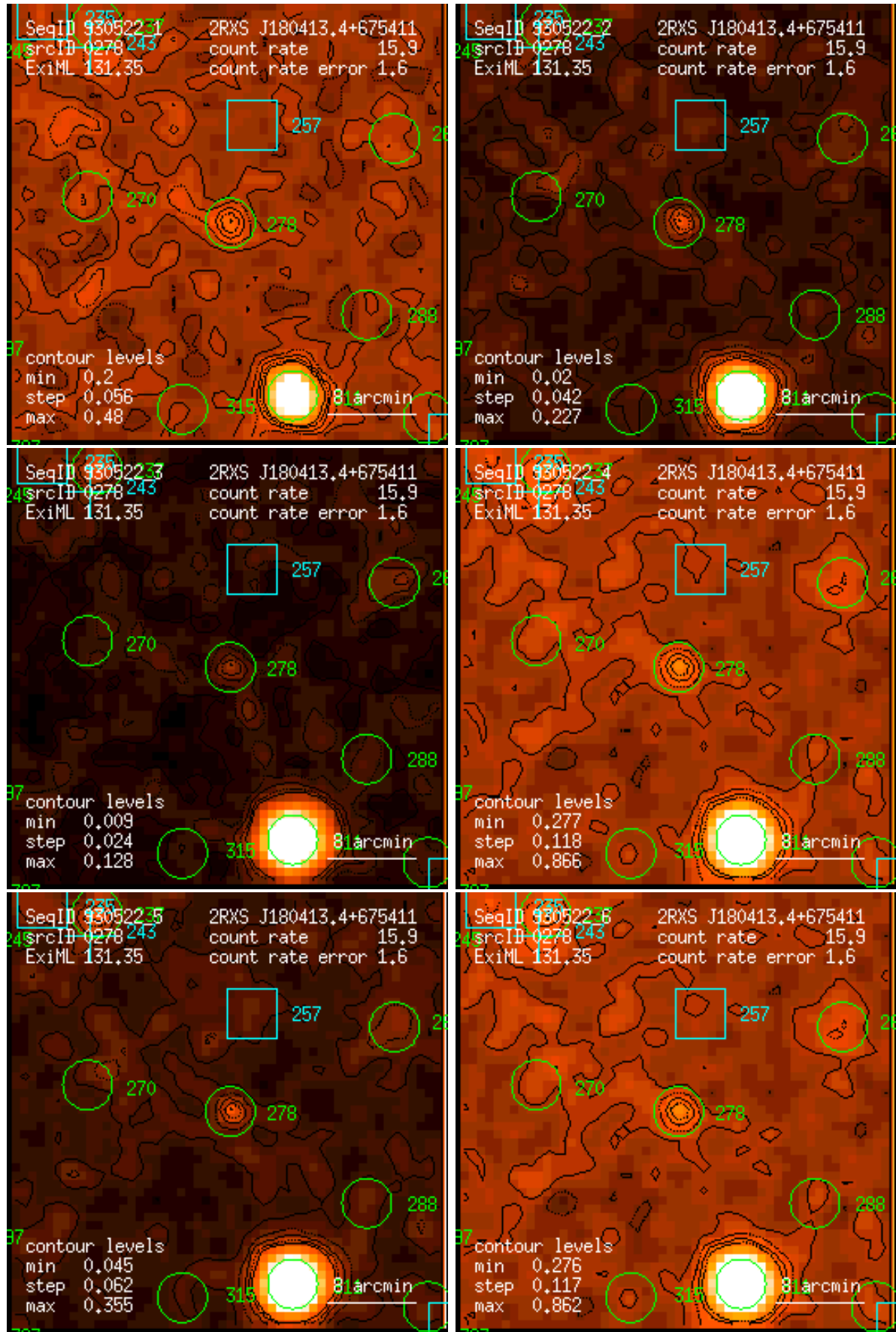
Figure 278: RASS 930522: detection 0278: band rate images, Gaussian filter: (1) PSPC channels 11 – 41, (2) 52 – 90, (3) 91 – 201, (4) 11 – 235, (5) 52 – 201, (6) 11 – 201. Broad band rates in counts/ks. Band rate contour levels in counts/ks/arcmin 2 .
