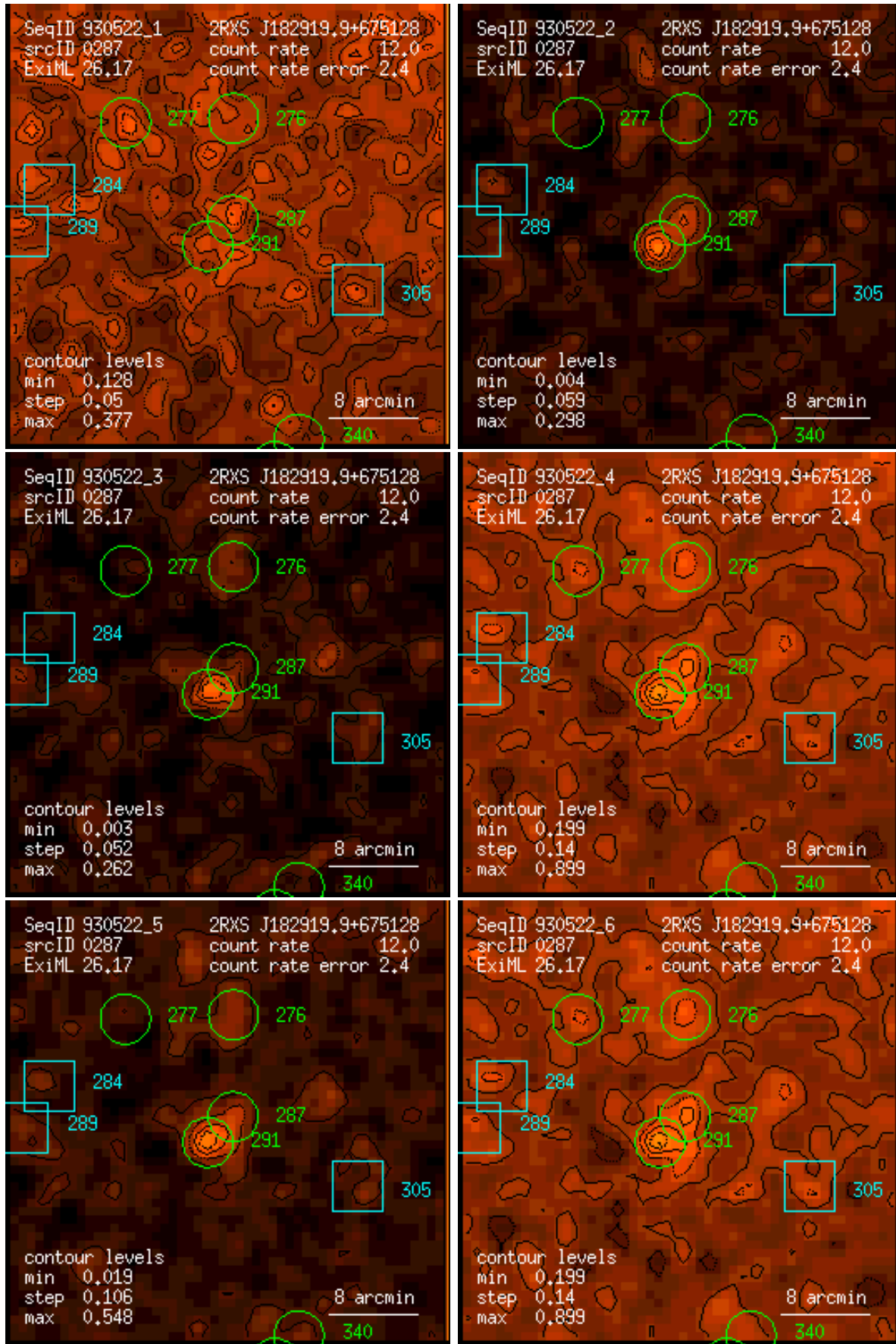
Figure 287: RASS 930522: detection 0287: band rate images, Gaussian filter: (1) PSPC channels 11 – 41, (2) 52 – 90, (3) 91 – 201, (4) 11 – 235, (5) 52 – 201, (6) 11 – 201. Broad band rates in counts/ks. Band rate contour levels in counts/ks/arcmin 2 .
