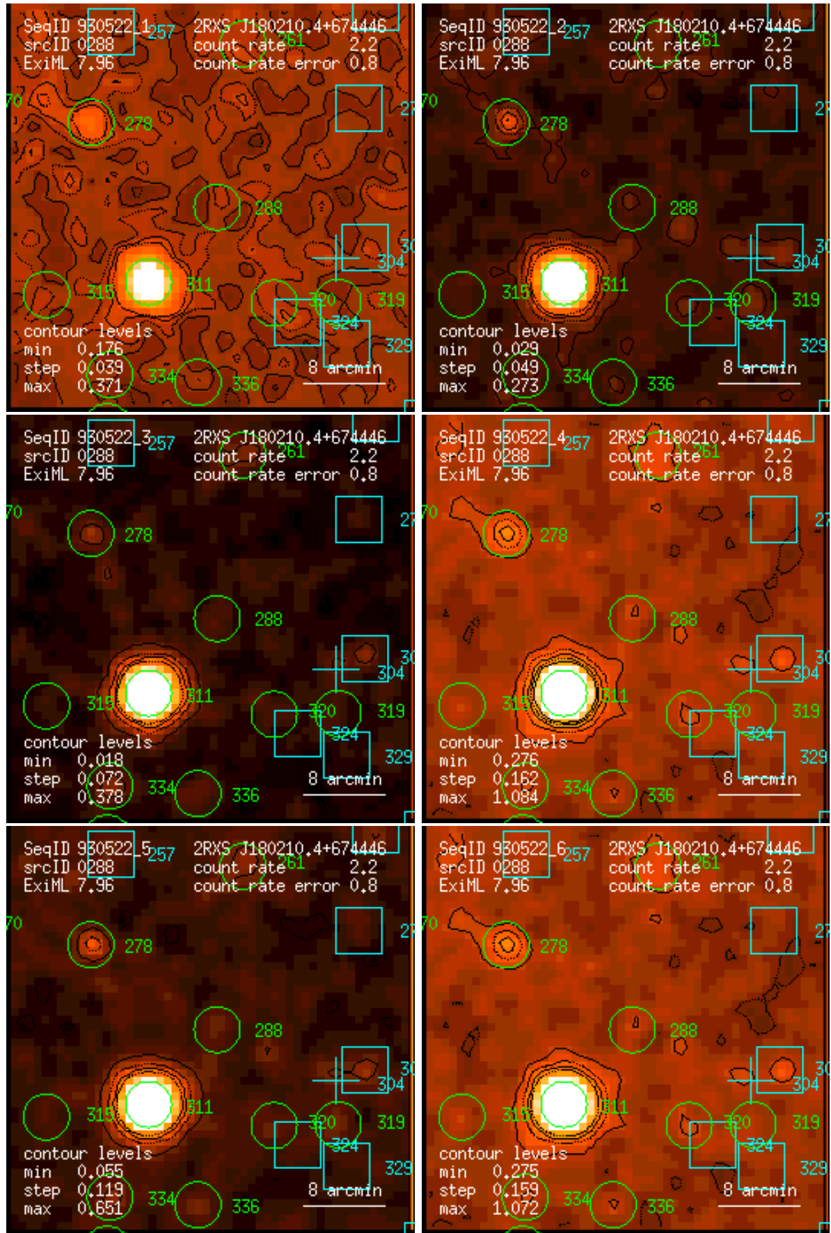
Figure 288: RASS 930522: detection 0288: band rate images, Gaussian filter: (1) PSPC channels 11 – 41, (2) 52 – 90, (3) 91 – 201, (4) 11 – 235, (5) 52 – 201, (6) 11 – 201. Broad band rates in counts/ks. Band rate contour levels in counts/ks/arcmin 2 .
