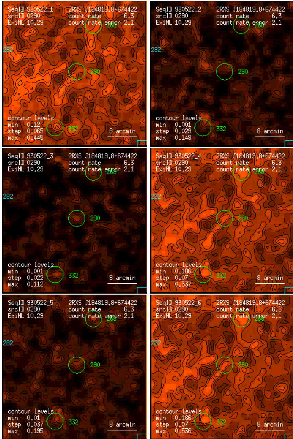
Figure 290: RASS 930522: detection 0290: band rate images, Gaussian filter: (1) PSPC channels 11 – 41, (2) 52 – 90, (3) 91 – 201, (4) 11 – 235, (5) 52 – 201, (6) 11 – 201. Broad band rates in counts/ks. Band rate contour levels in counts/ks/arcmin 2 .
