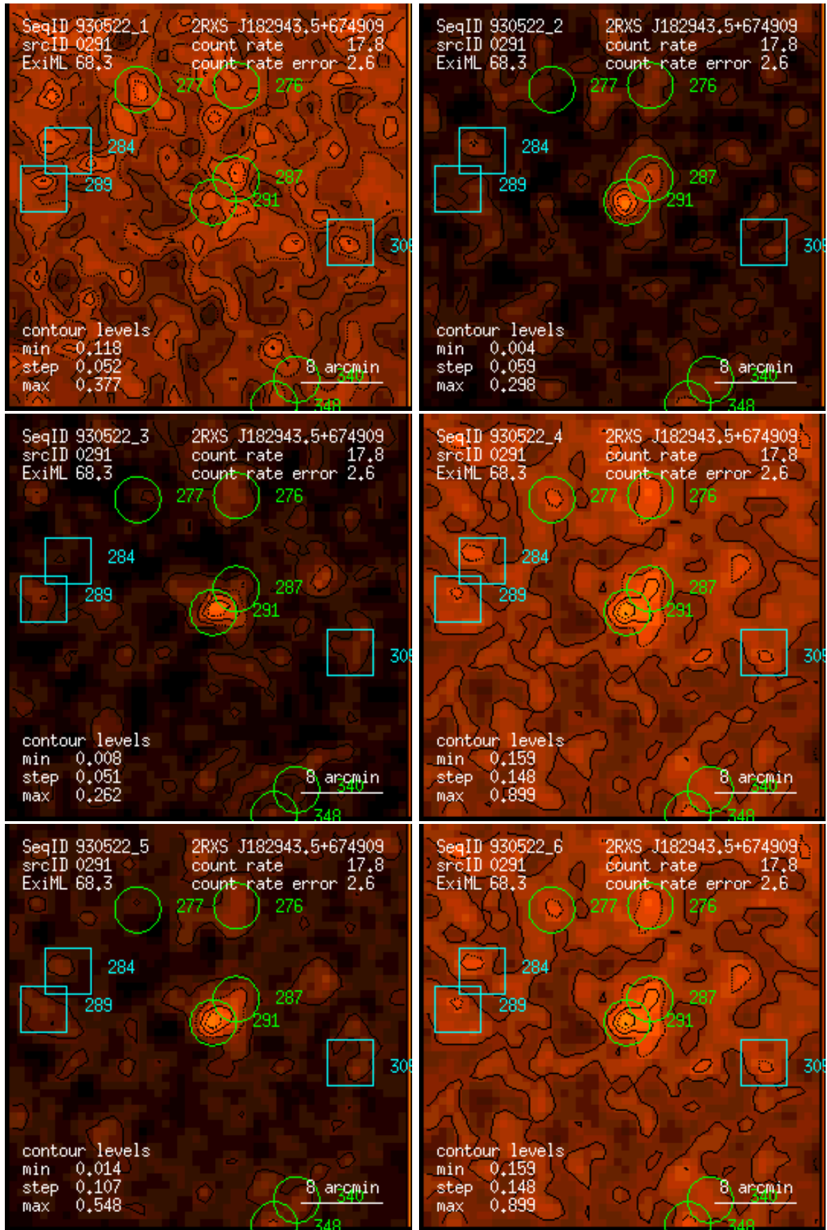
Figure 291: RASS 930522: detection 0291: band rate images, Gaussian filter: (1) PSPC channels 11 – 41, (2) 52 – 90, (3) 91 – 201, (4) 11 – 235, (5) 52 – 201, (6) 11 – 201. Broad band rates in counts/ks. Band rate contour levels in counts/ks/arcmin 2 .
