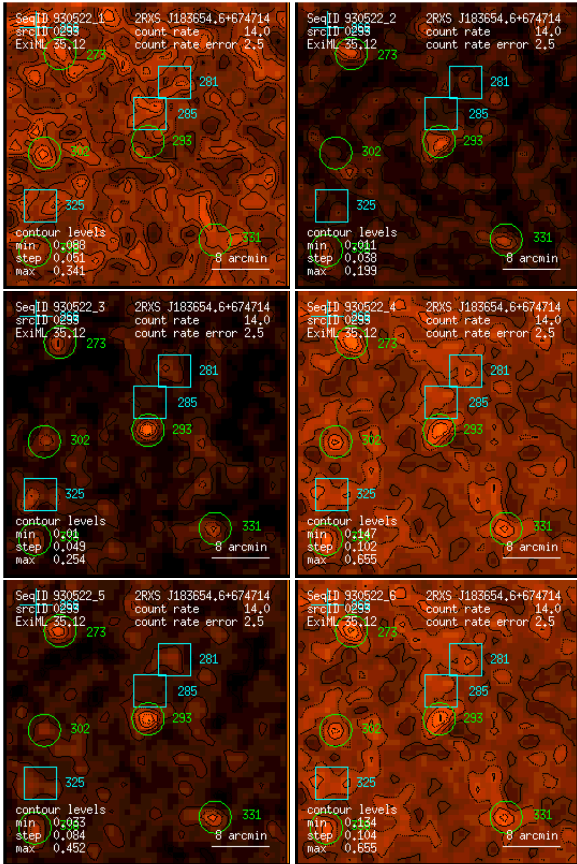
Figure 293: RASS 930522: detection 0293: band rate images, Gaussian filter: (1) PSPC channels 11 – 41, (2) 52 – 90, (3) 91 – 201, (4) 11 – 235, (5) 52 – 201, (6) 11 – 201. Broad band rates in counts/ks. Band rate contour levels in counts/ks/arcmin 2 .
