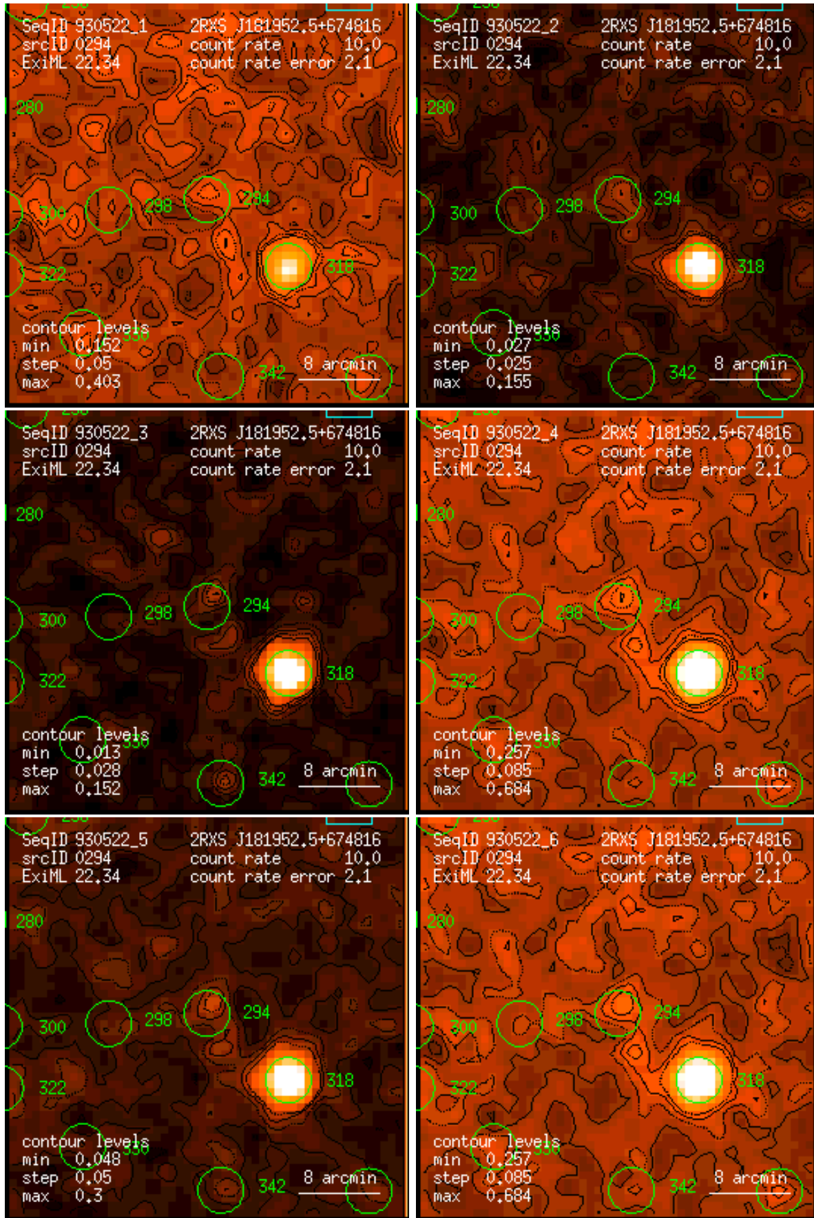
Figure 294: RASS 930522: detection 0294: band rate images, Gaussian filter: (1) PSPC channels 11 – 41, (2) 52 – 90, (3) 91 – 201, (4) 11 – 235, (5) 52 – 201, (6) 11 – 201. Broad band rates in counts/ks. Band rate contour levels in counts/ks/arcmin 2 .
