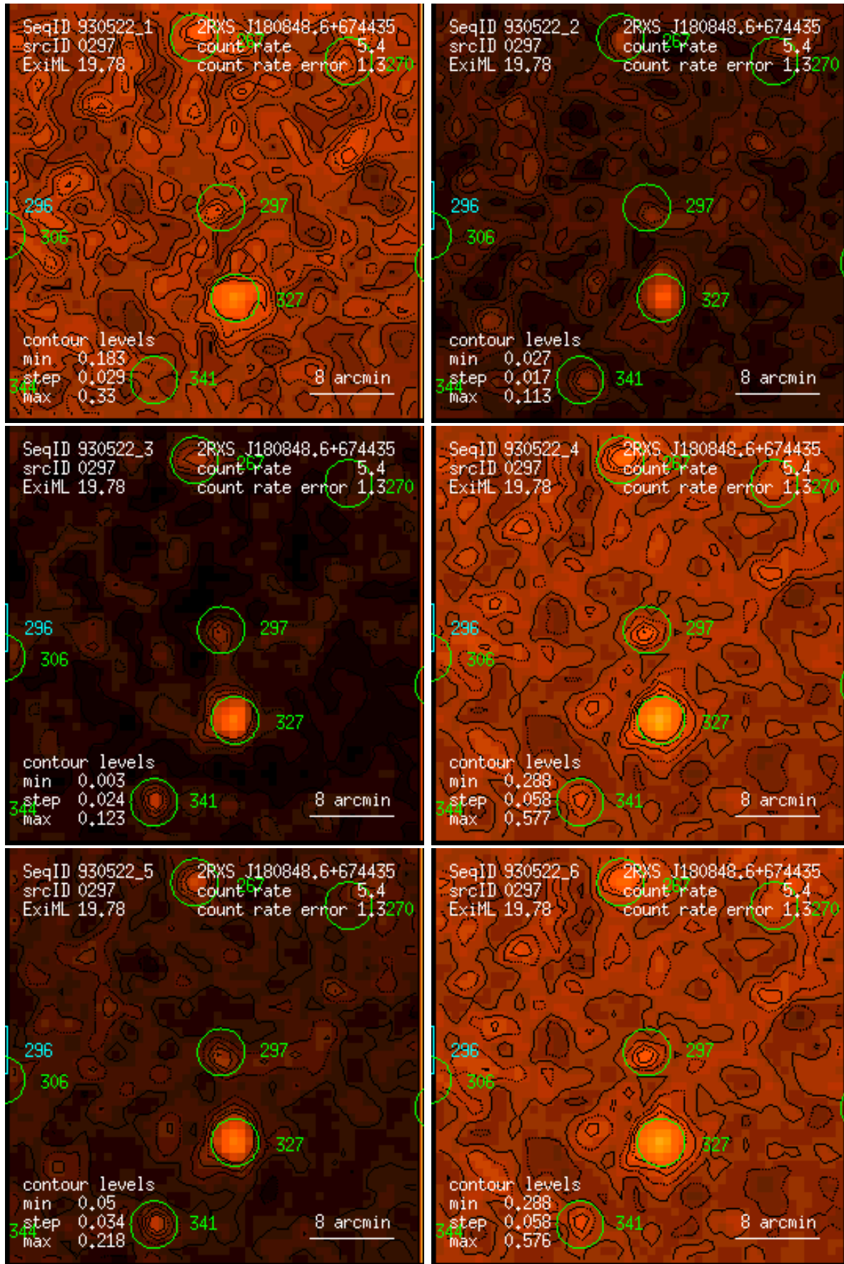
Figure 297: RASS 930522: detection 0297: band rate images, Gaussian filter: (1) PSPC channels 11 – 41, (2) 52 – 90, (3) 91 – 201, (4) 11 – 235, (5) 52 – 201, (6) 11 – 201. Broad band rates in counts/ks. Band rate contour levels in counts/ks/arcmin 2 .
