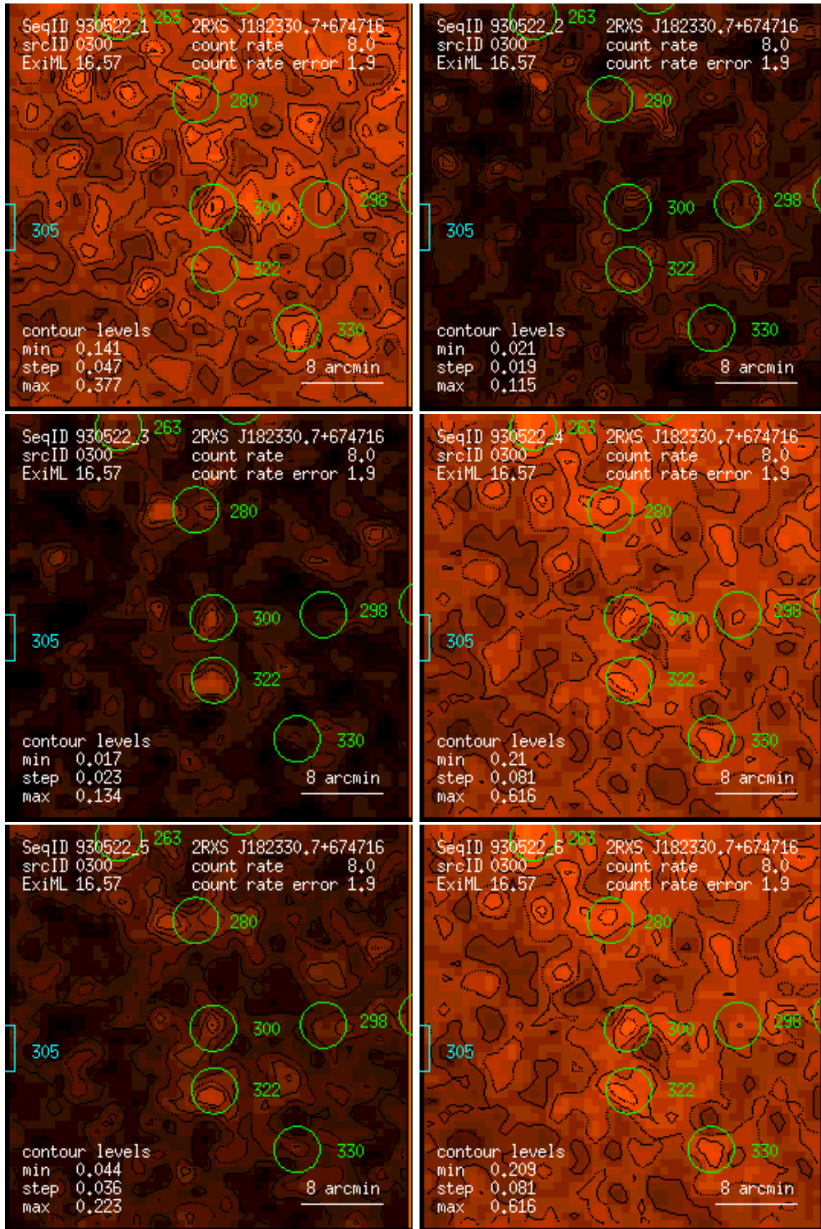
Figure 300: RASS 930522: detection 0300: band rate images, Gaussian filter: (1) PSPC channels 11 – 41, (2) 52 – 90, (3) 91 – 201, (4) 11 – 235, (5) 52 – 201, (6) 11 – 201. Broad band rates in counts/ks. Band rate contour levels in counts/ks/arcmin 2 .
