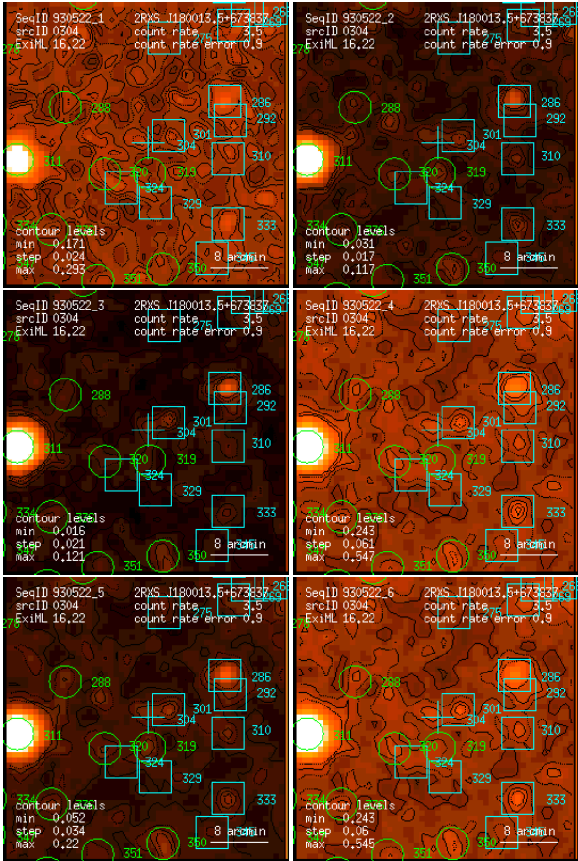
Figure 304: RASS 930522: detection 0304: band rate images, Gaussian filter: (1) PSPC channels 11 – 41, (2) 52 – 90, (3) 91 – 201, (4) 11 – 235, (5) 52 – 201, (6) 11 – 201. Broad band rates in counts/ks. Band rate contour levels in counts/ks/arcmin 2 .
