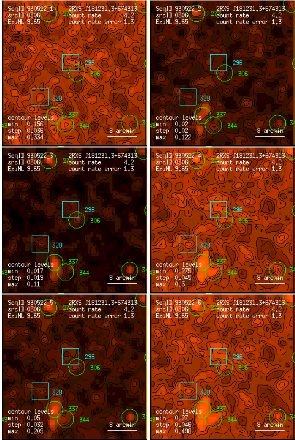
Figure 306: RASS 930522: detection 0306: band rate images, Gaussian filter: (1) PSPC channels 11 – 41, (2) 52 – 90, (3) 91 – 201, (4) 11 – 235, (5) 52 – 201, (6) 11 – 201. Broad band rates in counts/ks. Band rate contour levels in counts/ks/arcmin 2 .
