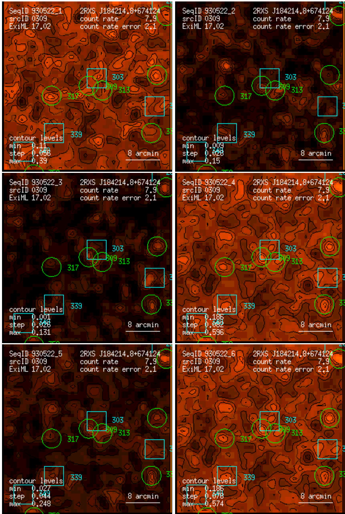
Figure 309: RASS 930522: detection 0309: band rate images, Gaussian filter: (1) PSPC channels 11 – 41, (2) 52 – 90, (3) 91 – 201, (4) 11 – 235, (5) 52 – 201, (6) 11 – 201. Broad band rates in counts/ks. Band rate contour levels in counts/ks/arcmin 2 .
