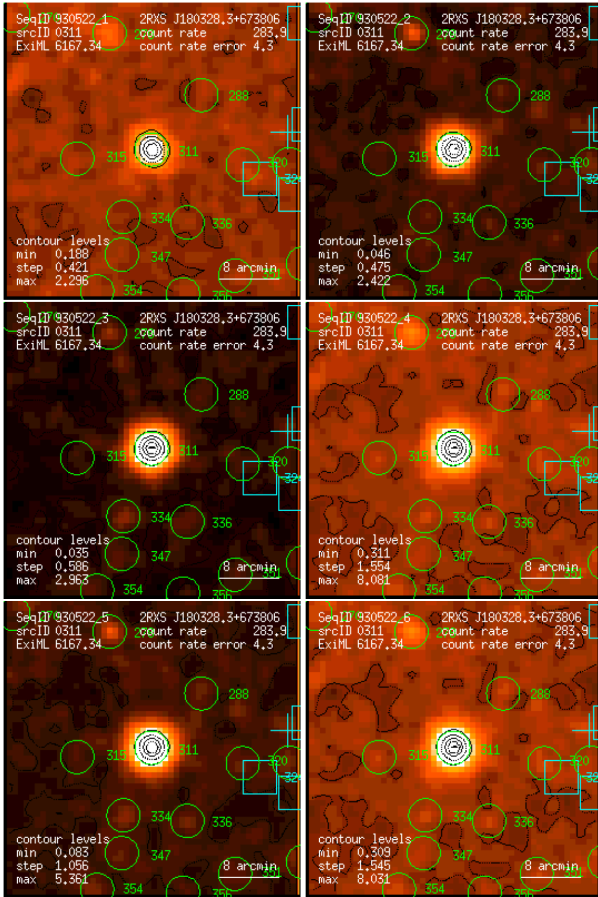
Figure 311: RASS 930522: detection 0311: band rate images, Gaussian filter: (1) PSPC channels 11 – 41, (2) 52 – 90, (3) 91 – 201, (4) 11 – 235, (5) 52 – 201, (6) 11 – 201. Broad band rates in counts/ks. Band rate contour levels in counts/ks/arcmin 2 .
