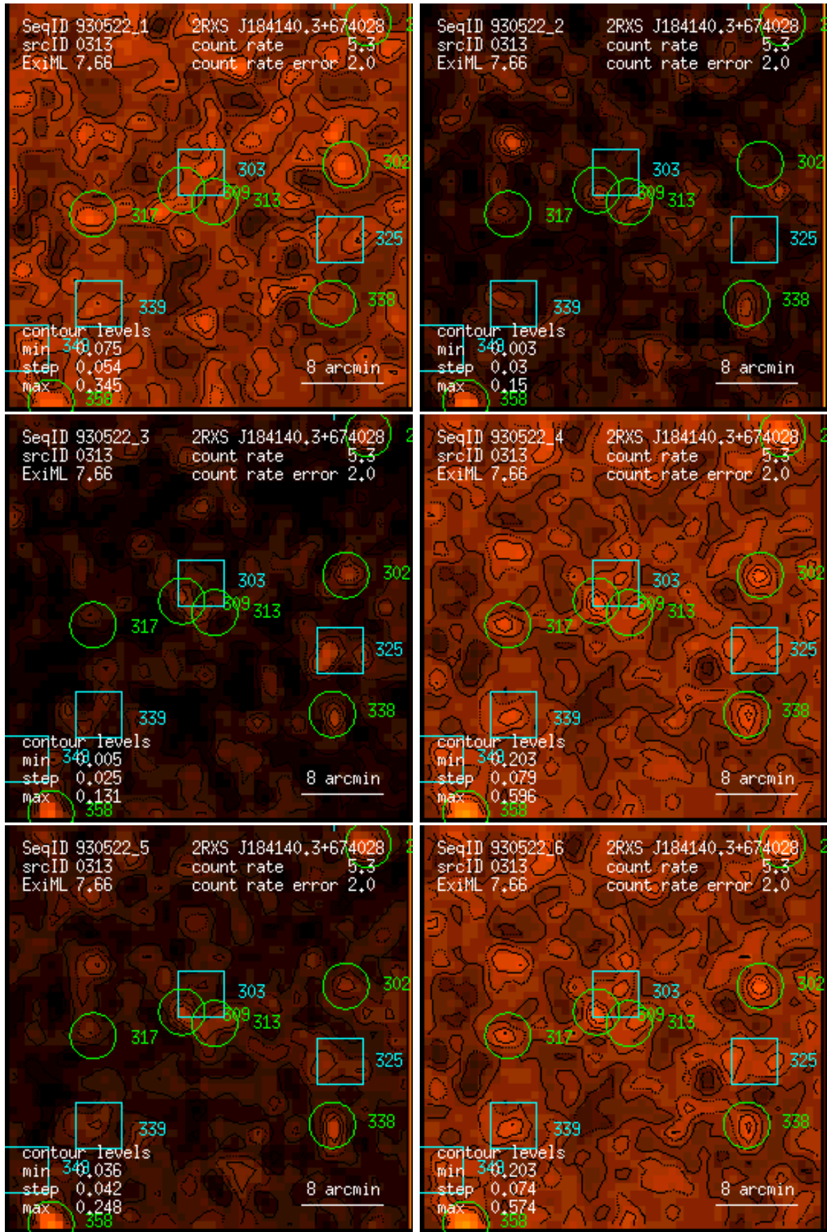
Figure 313: RASS 930522: detection 0313: band rate images, Gaussian filter: (1) PSPC channels 11 – 41, (2) 52 – 90, (3) 91 – 201, (4) 11 – 235, (5) 52 – 201, (6) 11 – 201. Broad band rates in counts/ks. Band rate contour levels in counts/ks/arcmin 2 .
