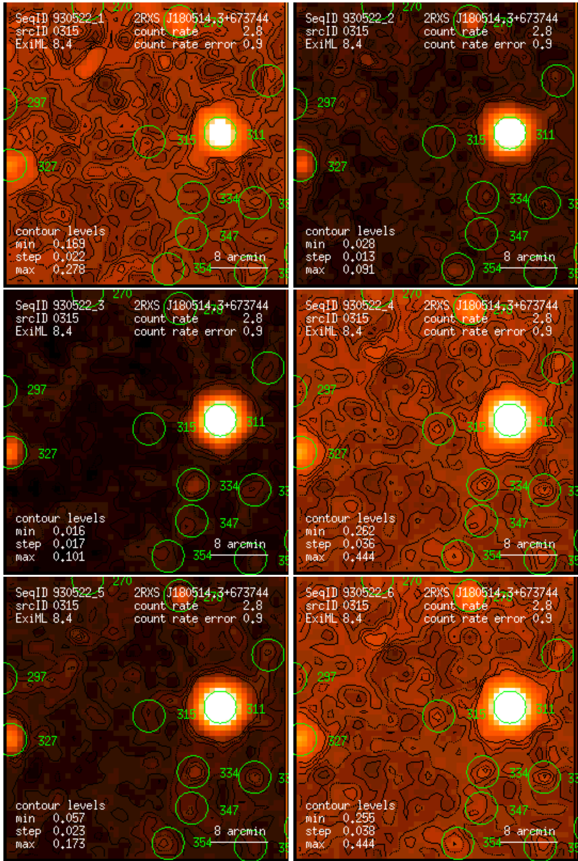
Figure 315: RASS 930522: detection 0315: band rate images, Gaussian filter: (1) PSPC channels 11 – 41, (2) 52 – 90, (3) 91 – 201, (4) 11 – 235, (5) 52 – 201, (6) 11 – 201. Broad band rates in counts/ks. Band rate contour levels in counts/ks/arcmin 2 .
