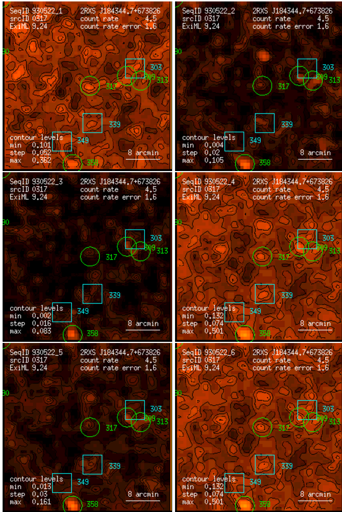
Figure 317: RASS 930522: detection 0317: band rate images, Gaussian filter: (1) PSPC channels 11 – 41, (2) 52 – 90, (3) 91 – 201, (4) 11 – 235, (5) 52 – 201, (6) 11 – 201. Broad band rates in counts/ks. Band rate contour levels in counts/ks/arcmin 2 .
