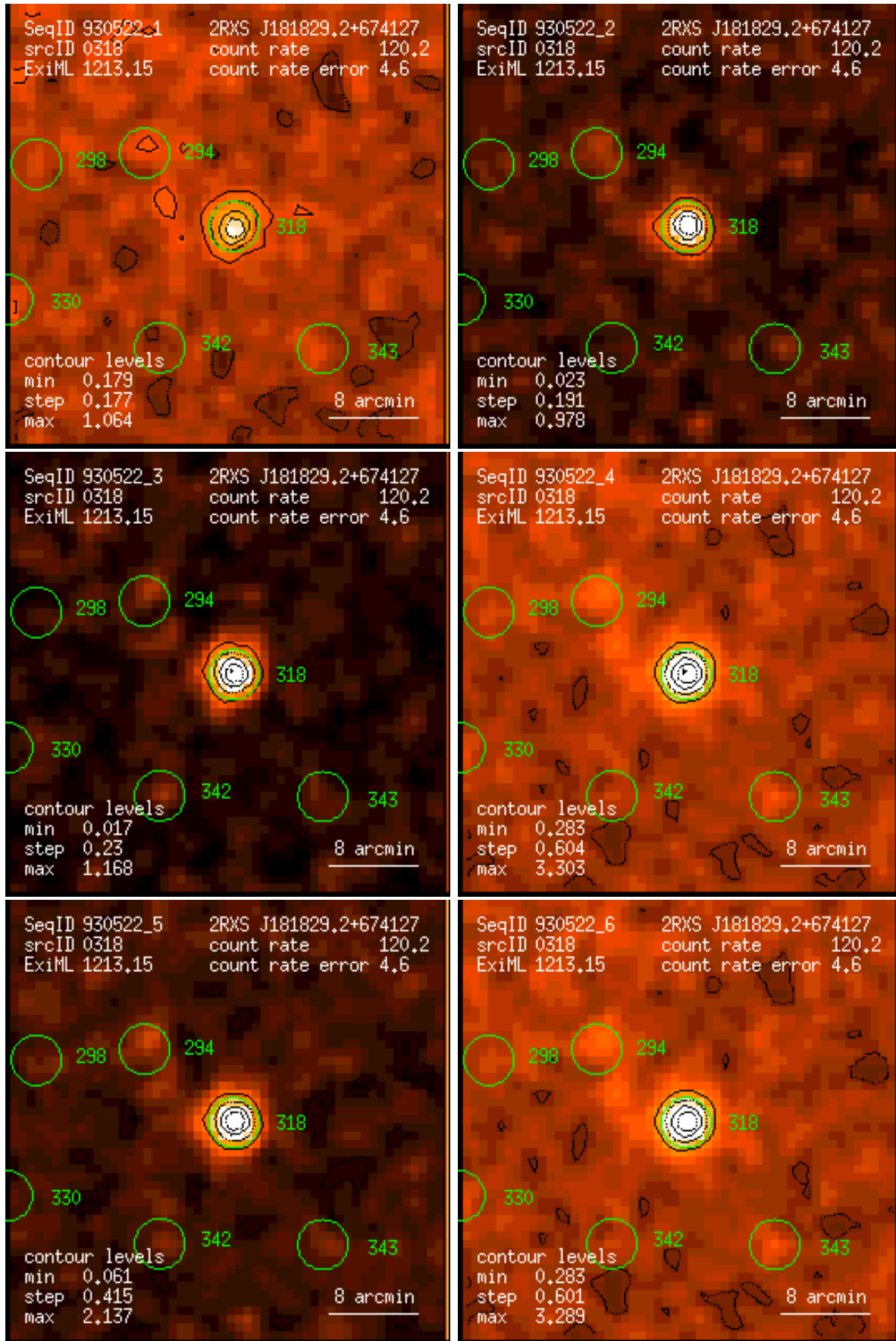
Figure 318: RASS 930522: detection 0318: band rate images, Gaussian filter: (1) PSPC channels 11 – 41, (2) 52 – 90, (3) 91 – 201, (4) 11 – 235, (5) 52 – 201, (6) 11 – 201. Broad band rates in counts/ks. Band rate contour levels in counts/ks/arcmin 2 .
