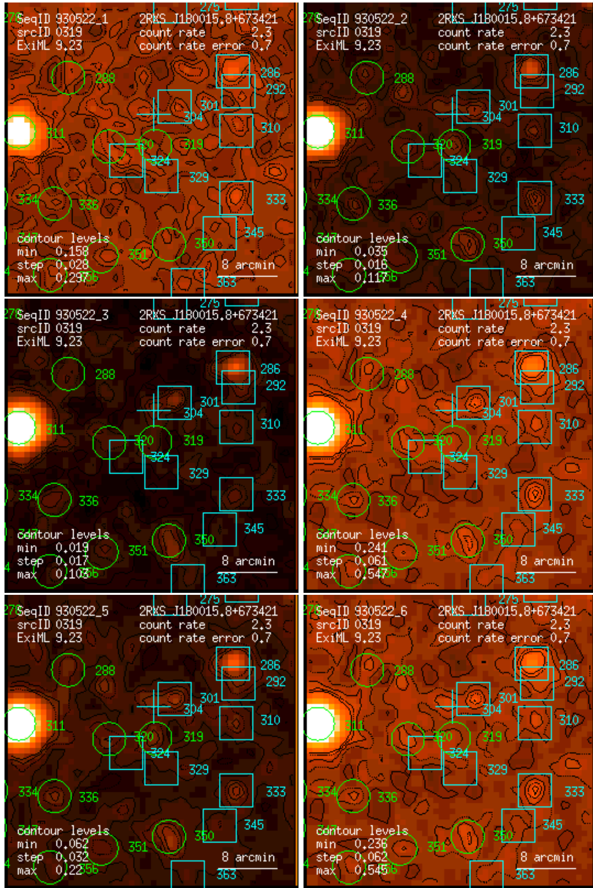
Figure 319: RASS 930522: detection 0319: band rate images, Gaussian filter: (1) PSPC channels 11 – 41, (2) 52 – 90, (3) 91 – 201, (4) 11 – 235, (5) 52 – 201, (6) 11 – 201. Broad band rates in counts/ks. Band rate contour levels in counts/ks/arcmin 2 .
