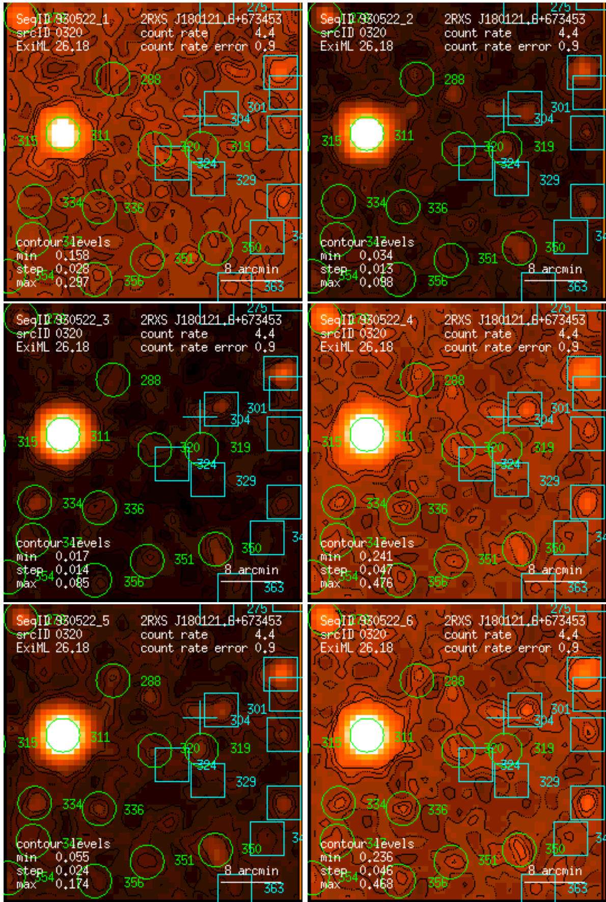
Figure 320: RASS 930522: detection 0320: band rate images, Gaussian filter: (1) PSPC channels 11 – 41, (2) 52 – 90, (3) 91 – 201, (4) 11 – 235, (5) 52 – 201, (6) 11 – 201. Broad band rates in counts/ks. Band rate contour levels in counts/ks/arcmin 2 .
