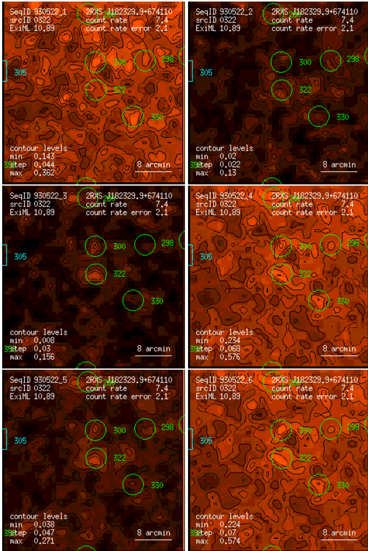
Figure 322: RASS 930522: detection 0322: band rate images, Gaussian filter: (1) PSPC channels 11 – 41, (2) 52 – 90, (3) 91 – 201, (4) 11 – 235, (5) 52 – 201, (6) 11 – 201. Broad band rates in counts/ks. Band rate contour levels in counts/ks/arcmin 2 .
