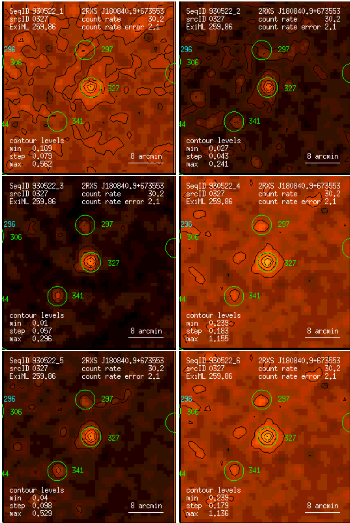
Figure 327: RASS 930522: detection 0327: band rate images, Gaussian filter: (1) PSPC channels 11 – 41, (2) 52 – 90, (3) 91 – 201, (4) 11 – 235, (5) 52 – 201, (6) 11 – 201. Broad band rates in counts/ks. Band rate contour levels in counts/ks/arcmin 2 .
