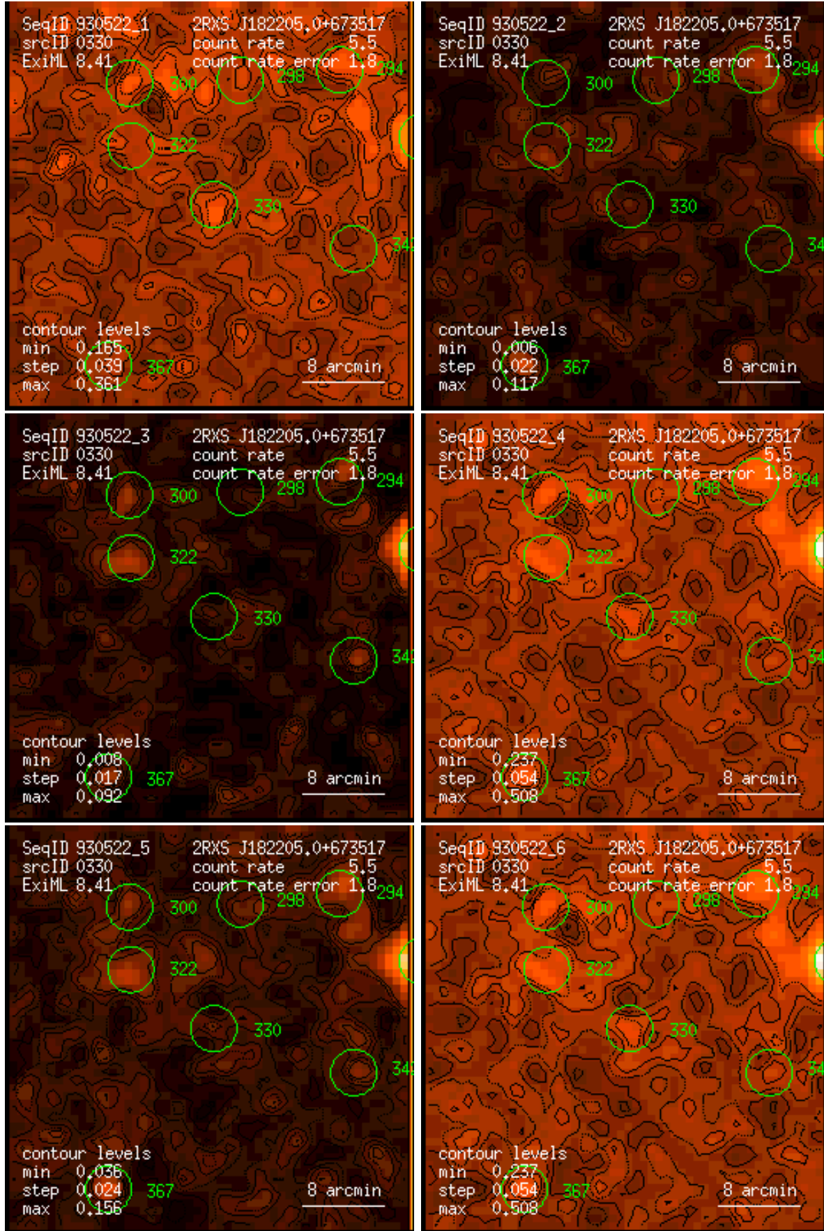
Figure 330: RASS 930522: detection 0330: band rate images, Gaussian filter: (1) PSPC channels 11 – 41, (2) 52 – 90, (3) 91 – 201, (4) 11 – 235, (5) 52 – 201, (6) 11 – 201. Broad band rates in counts/ks. Band rate contour levels in counts/ks/arcmin 2 .
