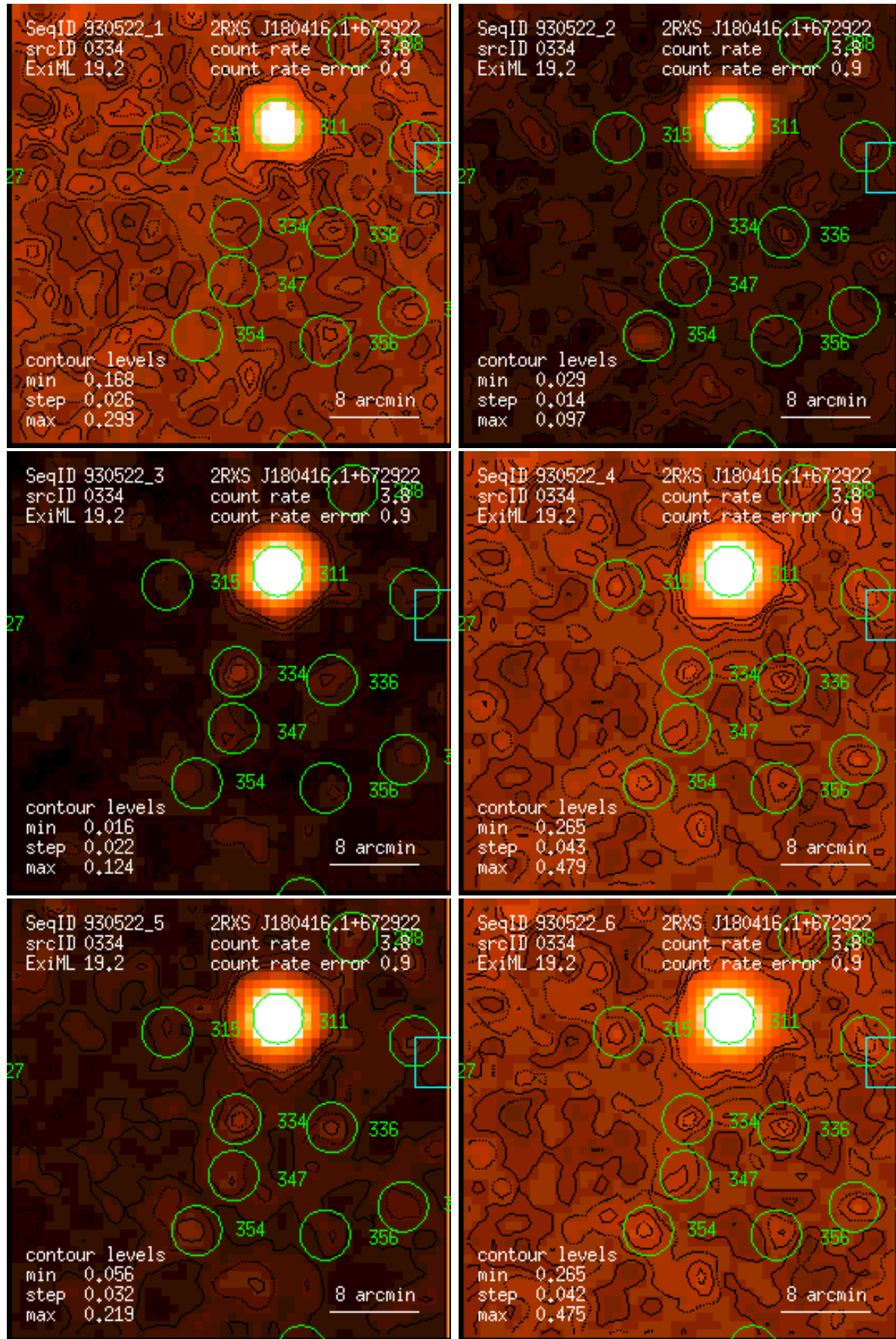
Figure 334: RASS 930522: detection 0334: band rate images, Gaussian filter: (1) PSPC channels 11 – 41, (2) 52 – 90, (3) 91 – 201, (4) 11 – 235, (5) 52 – 201, (6) 11 – 201. Broad band rates in counts/ks. Band rate contour levels in counts/ks/arcmin 2 .
