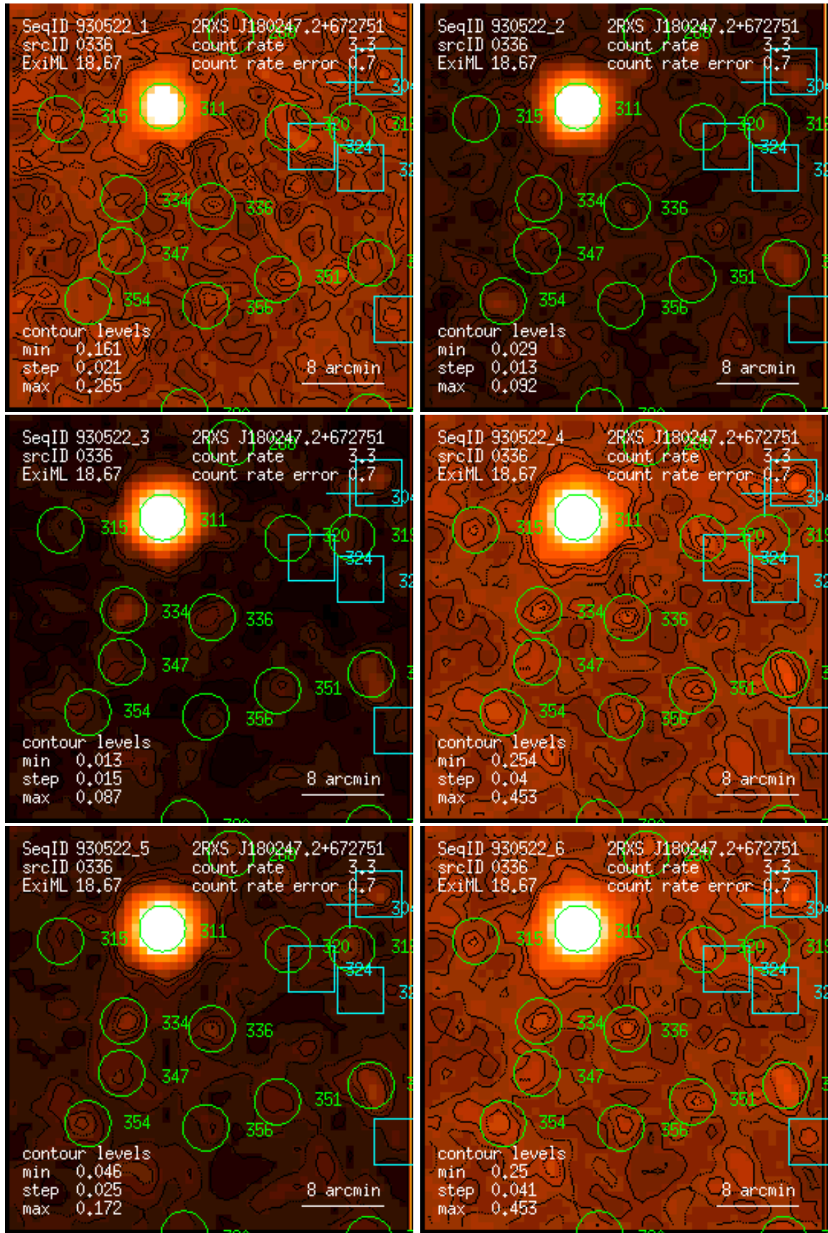
Figure 336: RASS 930522: detection 0336: band rate images, Gaussian filter: (1) PSPC channels 11 – 41, (2) 52 – 90, (3) 91 – 201, (4) 11 – 235, (5) 52 – 201, (6) 11 – 201. Broad band rates in counts/ks. Band rate contour levels in counts/ks/arcmin 2 .
