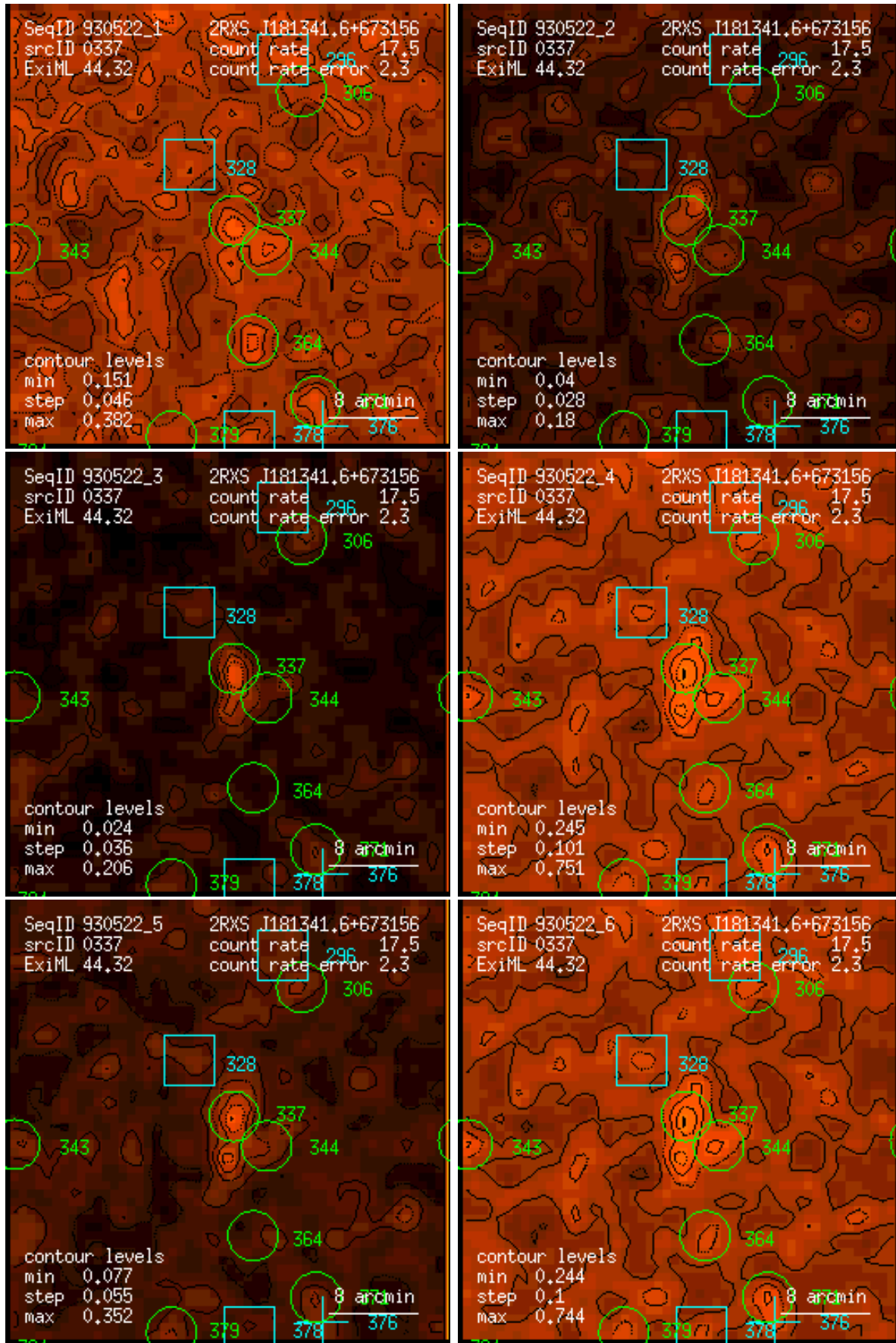
Figure 337: RASS 930522: detection 0337: band rate images, Gaussian filter: (1) PSPC channels 11 – 41, (2) 52 – 90, (3) 91 – 201, (4) 11 – 235, (5) 52 – 201, (6) 11 – 201. Broad band rates in counts/ks. Band rate contour levels in counts/ks/arcmin 2 .
