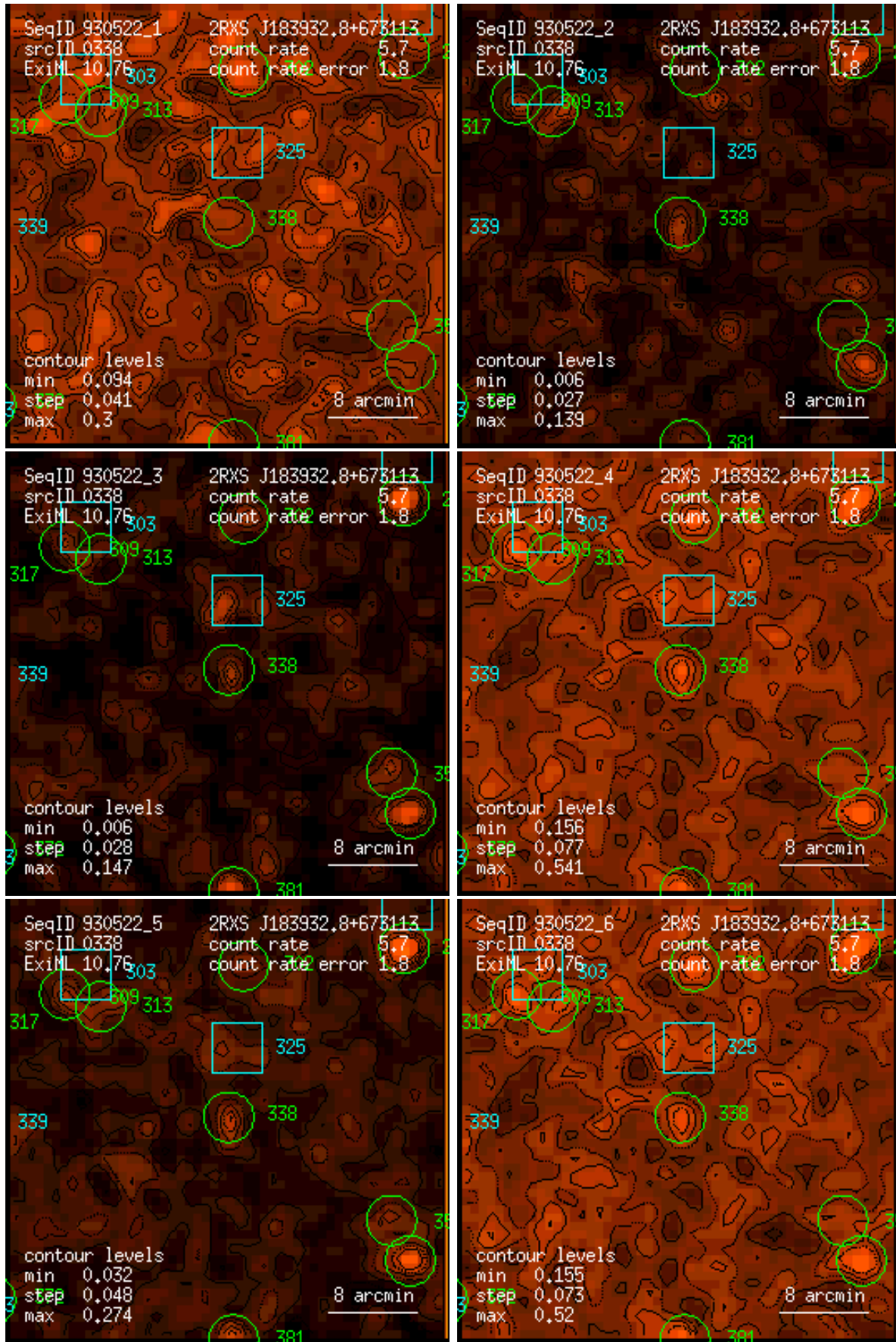
Figure 338: RASS 930522: detection 0338: band rate images, Gaussian filter: (1) PSPC channels 11 – 41, (2) 52 – 90, (3) 91 – 201, (4) 11 – 235, (5) 52 – 201, (6) 11 – 201. Broad band rates in counts/ks. Band rate contour levels in counts/ks/arcmin 2 .
