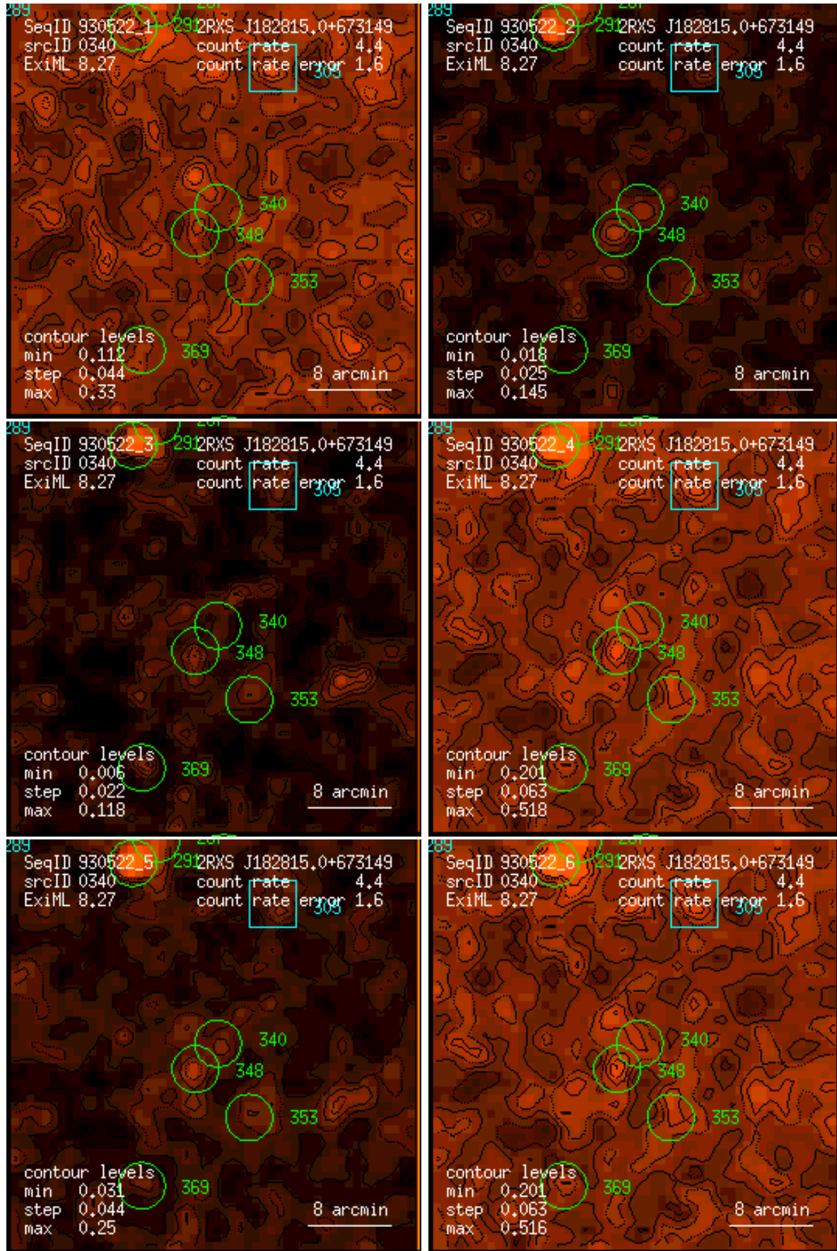
Figure 340: RASS 930522: detection 0340: band rate images, Gaussian filter: (1) PSPC channels 11 – 41, (2) 52 – 90, (3) 91 – 201, (4) 11 – 235, (5) 52 – 201, (6) 11 – 201. Broad band rates in counts/ks. Band rate contour levels in counts/ks/arcmin 2 .
