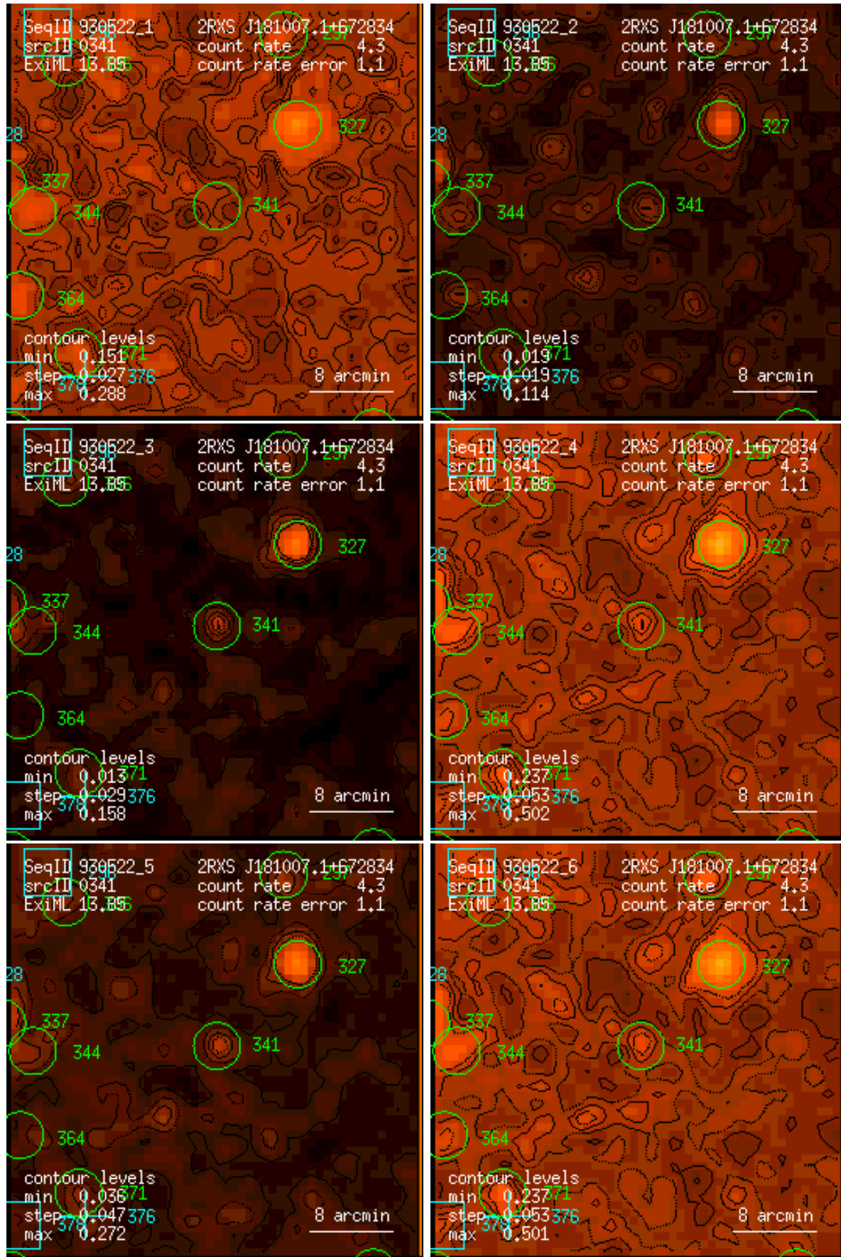
Figure 341: RASS 930522: detection 0341: band rate images, Gaussian filter: (1) PSPC channels 11 – 41, (2) 52 – 90, (3) 91 – 201, (4) 11 – 235, (5) 52 – 201, (6) 11 – 201. Broad band rates in counts/ks. Band rate contour levels in counts/ks/arcmin 2 .
