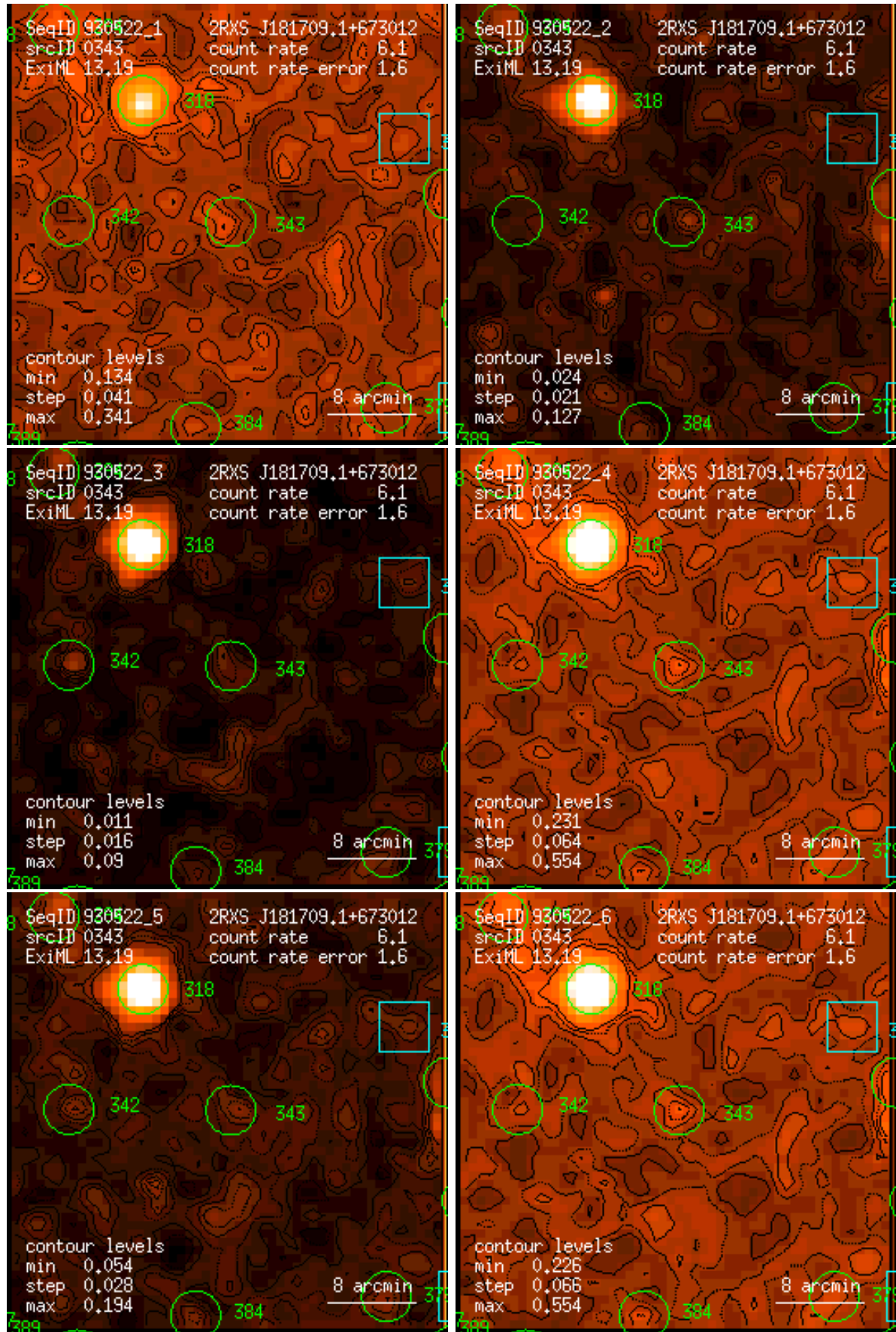
Figure 343: RASS 930522: detection 0343: band rate images, Gaussian filter: (1) PSPC channels 11 – 41, (2) 52 – 90, (3) 91 – 201, (4) 11 – 235, (5) 52 – 201, (6) 11 – 201. Broad band rates in counts/ks. Band rate contour levels in counts/ks/arcmin 2 .
