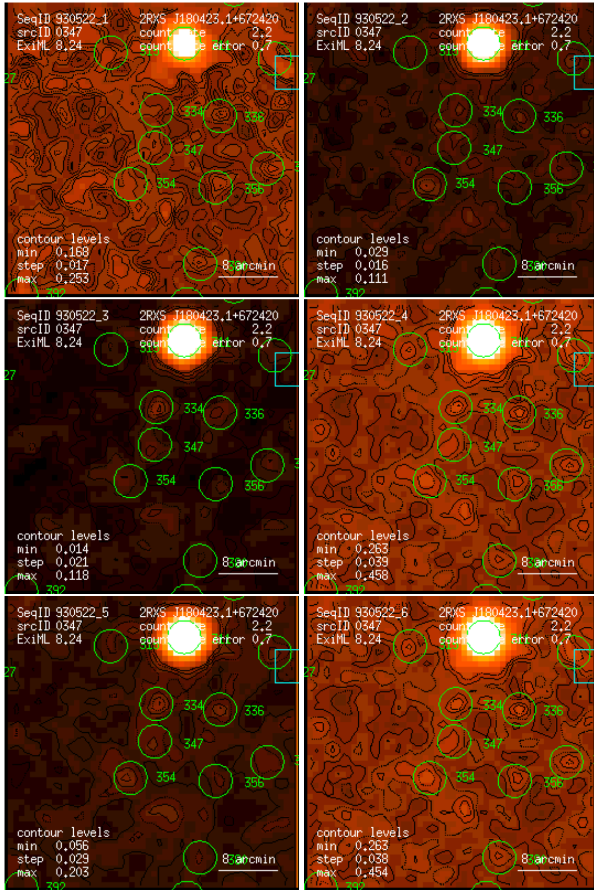
Figure 347: RASS 930522: detection 0347: band rate images, Gaussian filter: (1) PSPC channels 11 – 41, (2) 52 – 90, (3) 91 – 201, (4) 11 – 235, (5) 52 – 201, (6) 11 – 201. Broad band rates in counts/ks. Band rate contour levels in counts/ks/arcmin 2 .
