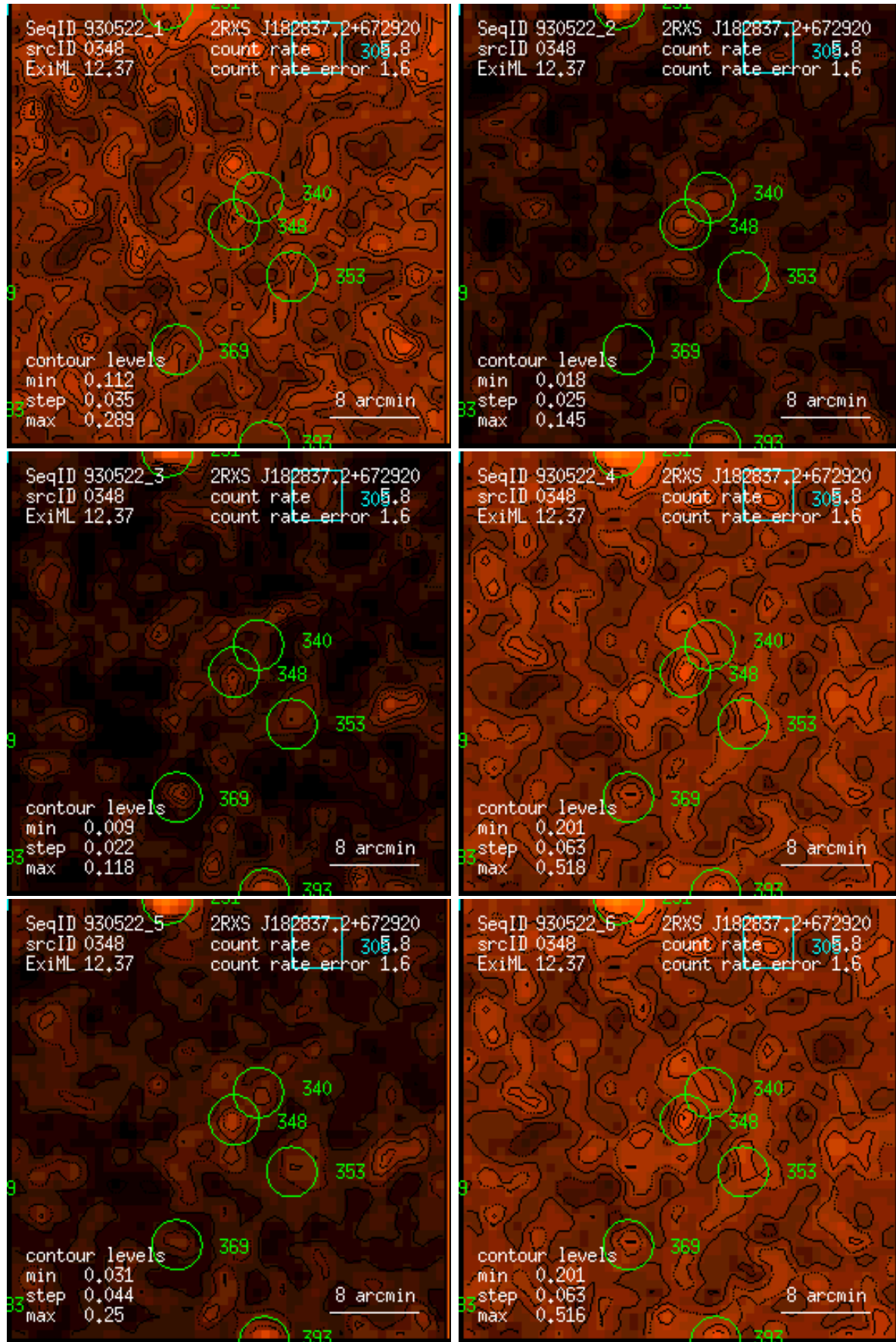
Figure 348: RASS 930522: detection 0348: band rate images, Gaussian filter: (1) PSPC channels 11 – 41, (2) 52 – 90, (3) 91 – 201, (4) 11 – 235, (5) 52 – 201, (6) 11 – 201. Broad band rates in counts/ks. Band rate contour levels in counts/ks/arcmin 2 .
