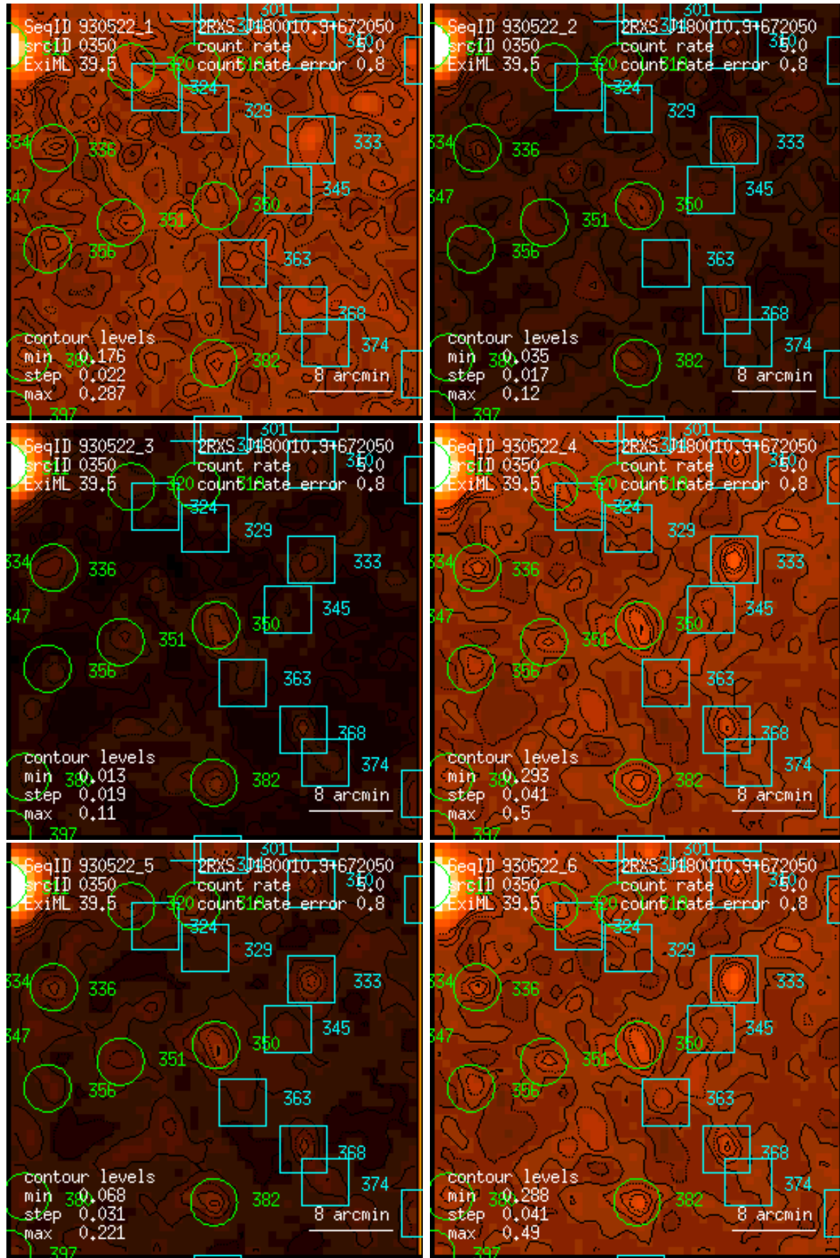
Figure 350: RASS 930522: detection 0350: band rate images, Gaussian filter: (1) PSPC channels 11 – 41, (2) 52 – 90, (3) 91 – 201, (4) 11 – 235, (5) 52 – 201, (6) 11 – 201. Broad band rates in counts/ks. Band rate contour levels in counts/ks/arcmin 2 .
