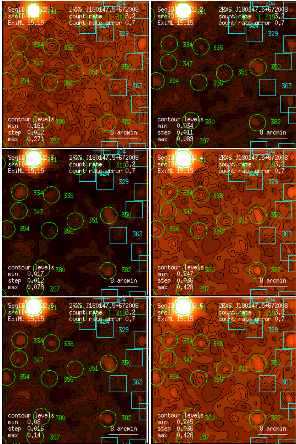
Figure 351: RASS 930522: detection 0351: band rate images, Gaussian filter: (1) PSPC channels 11 – 41, (2) 52 – 90, (3) 91 – 201, (4) 11 – 235, (5) 52 – 201, (6) 11 – 201. Broad band rates in counts/ks. Band rate contour levels in counts/ks/arcmin 2 .
