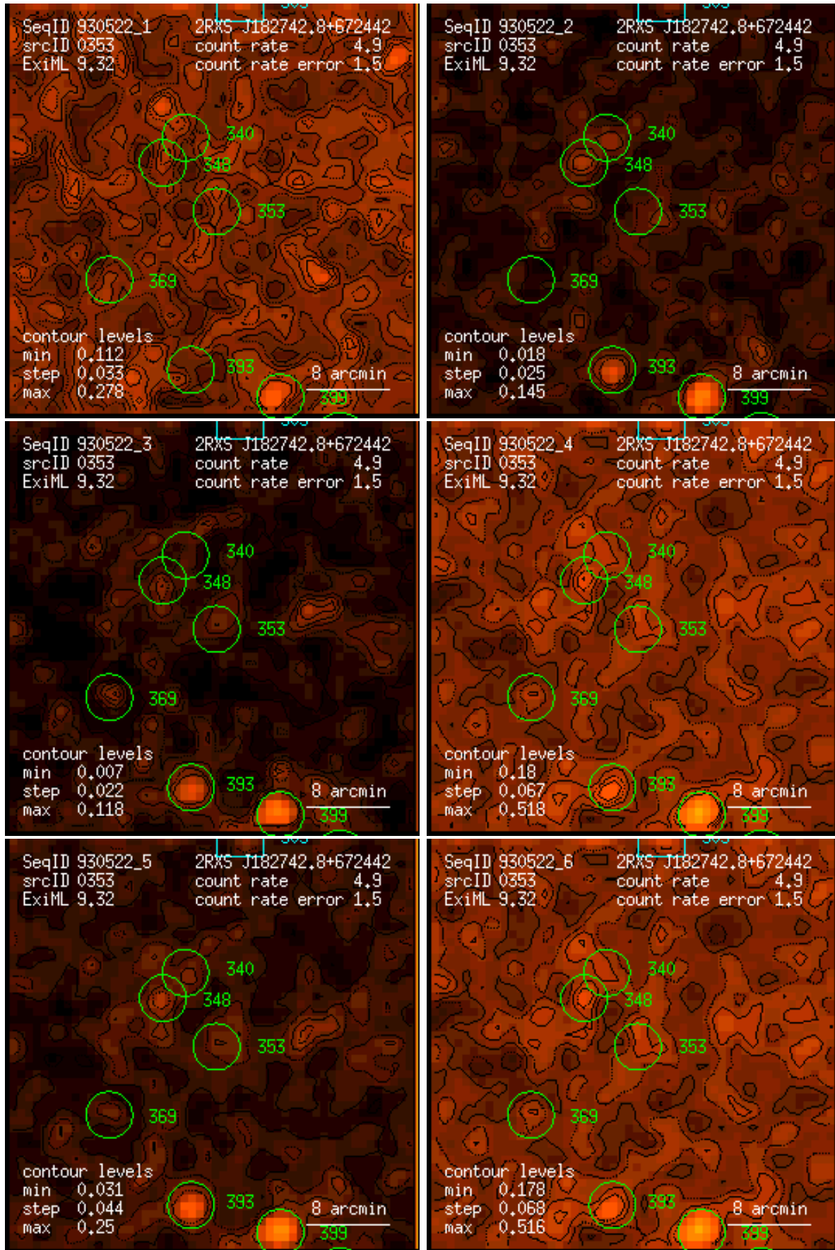
Figure 353: RASS 930522: detection 0353: band rate images, Gaussian filter: (1) PSPC channels 11 – 41, (2) 52 – 90, (3) 91 – 201, (4) 11 – 235, (5) 52 – 201, (6) 11 – 201. Broad band rates in counts/ks. Band rate contour levels in counts/ks/arcmin 2 .
