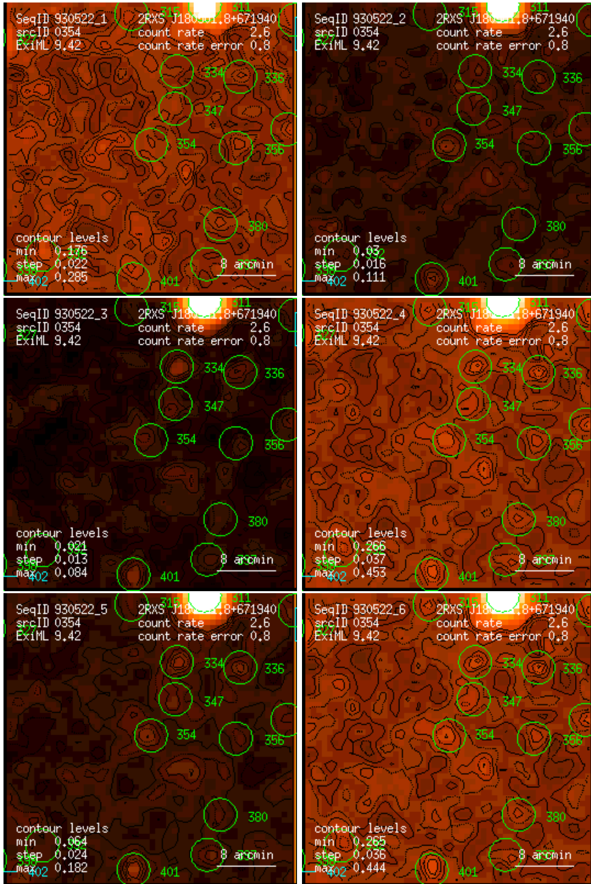
Figure 354: RASS 930522: detection 0354: band rate images, Gaussian filter: (1) PSPC channels 11 – 41, (2) 52 – 90, (3) 91 – 201, (4) 11 – 235, (5) 52 – 201, (6) 11 – 201. Broad band rates in counts/ks. Band rate contour levels in counts/ks/arcmin 2 .
